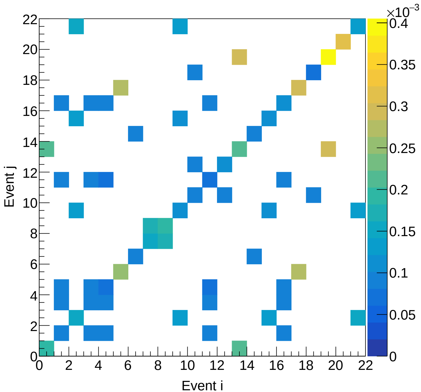
LH2 (mix) Covariance | M: [3.9, 4.2) xF: [0.75, 0.80)
