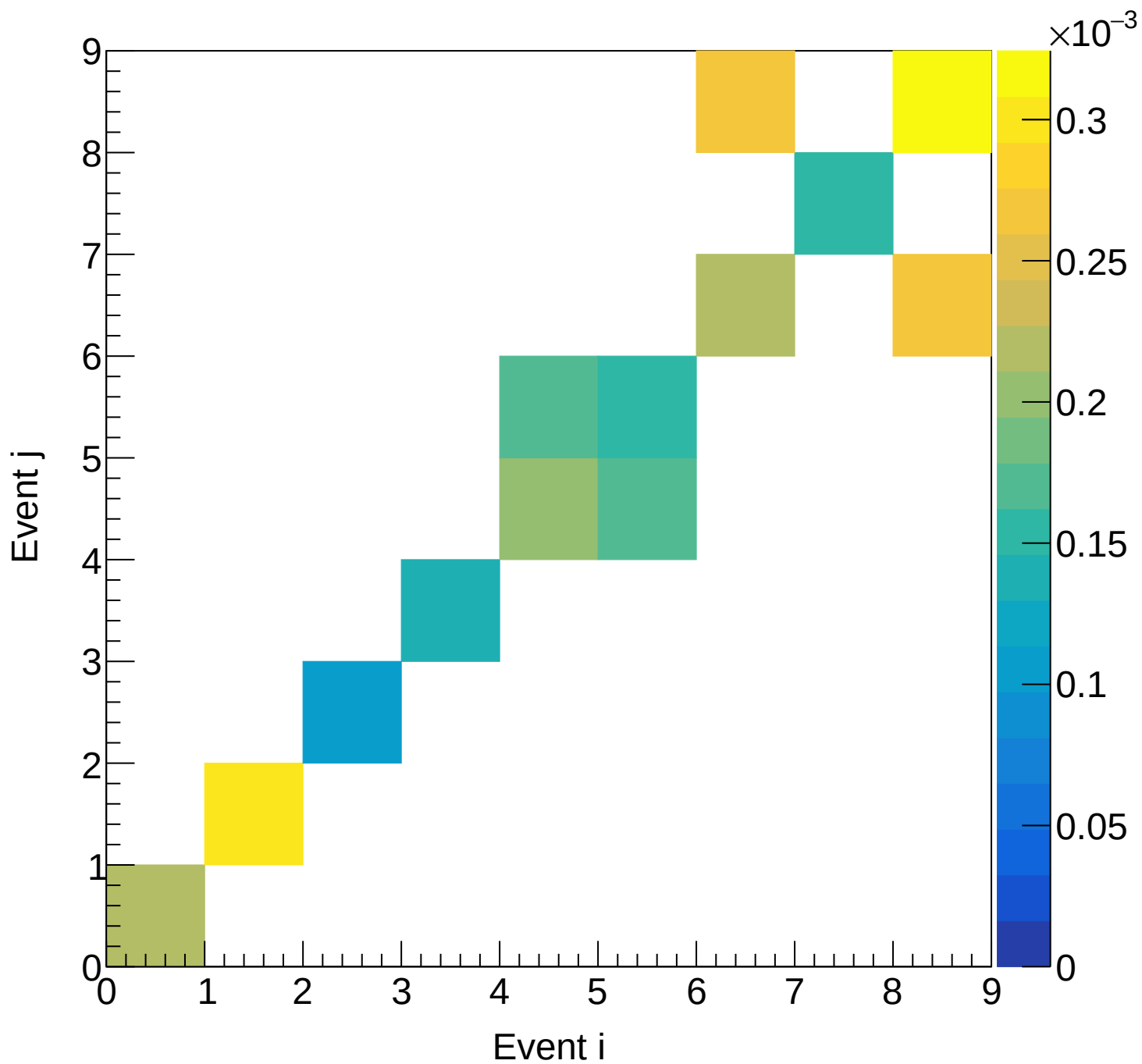
LH2 (mix) Covariance | M: [4.2, 4.5] xF: [0.75, 0.80]
