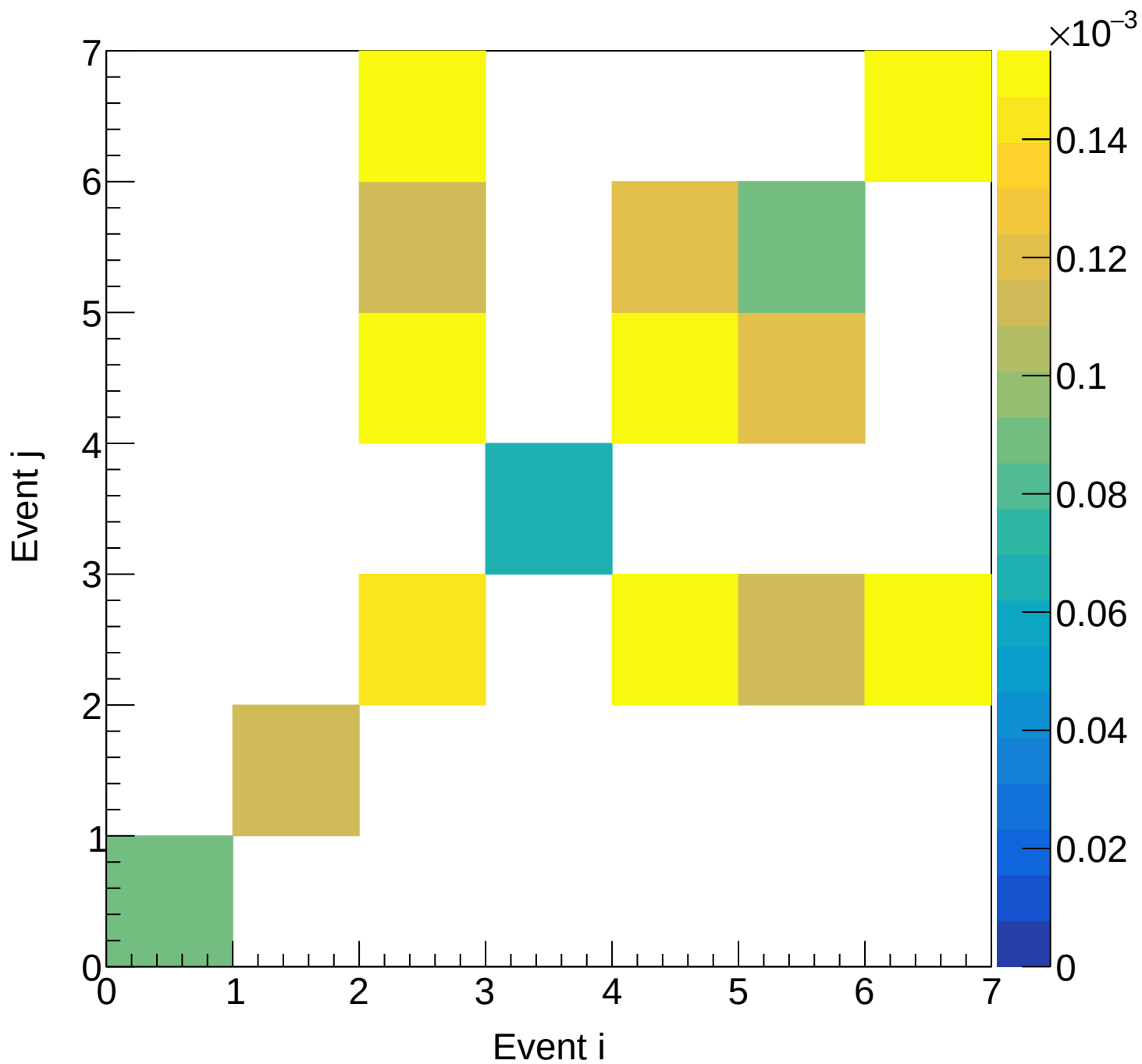
LH2 (mix) Covariance | M: [4.5, 4.8] xF: [0.75, 0.80]
