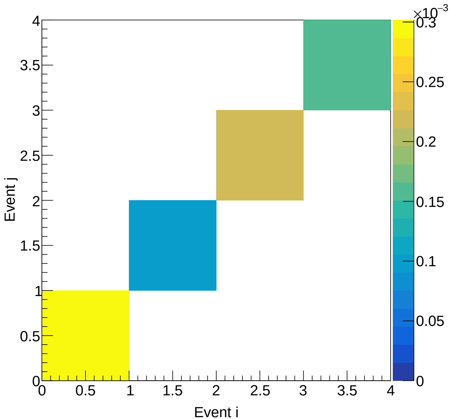
LH2 (mix) Covariance | M: [4.2, 4.5) xF: [0.80, 0.85)
