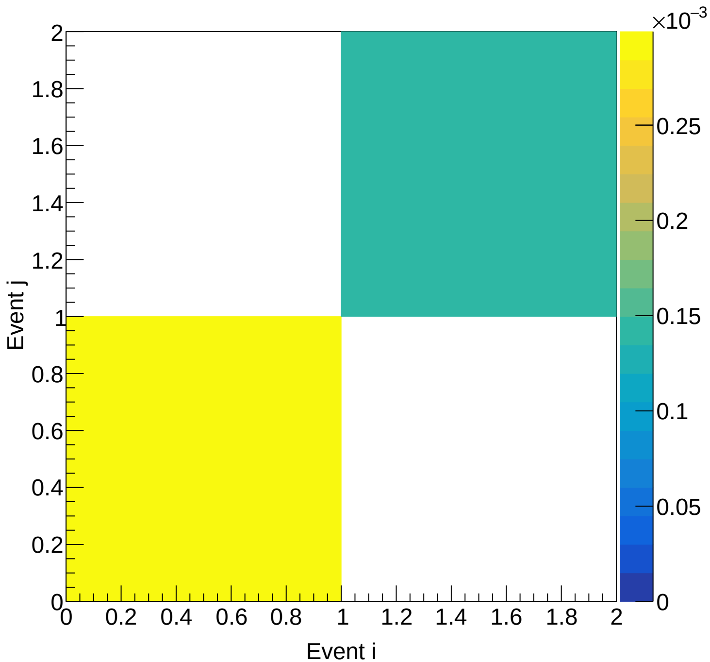
LH2 (mix) Covariance | M: [4.5, 4.8) xF: [0.80, 0.85)
