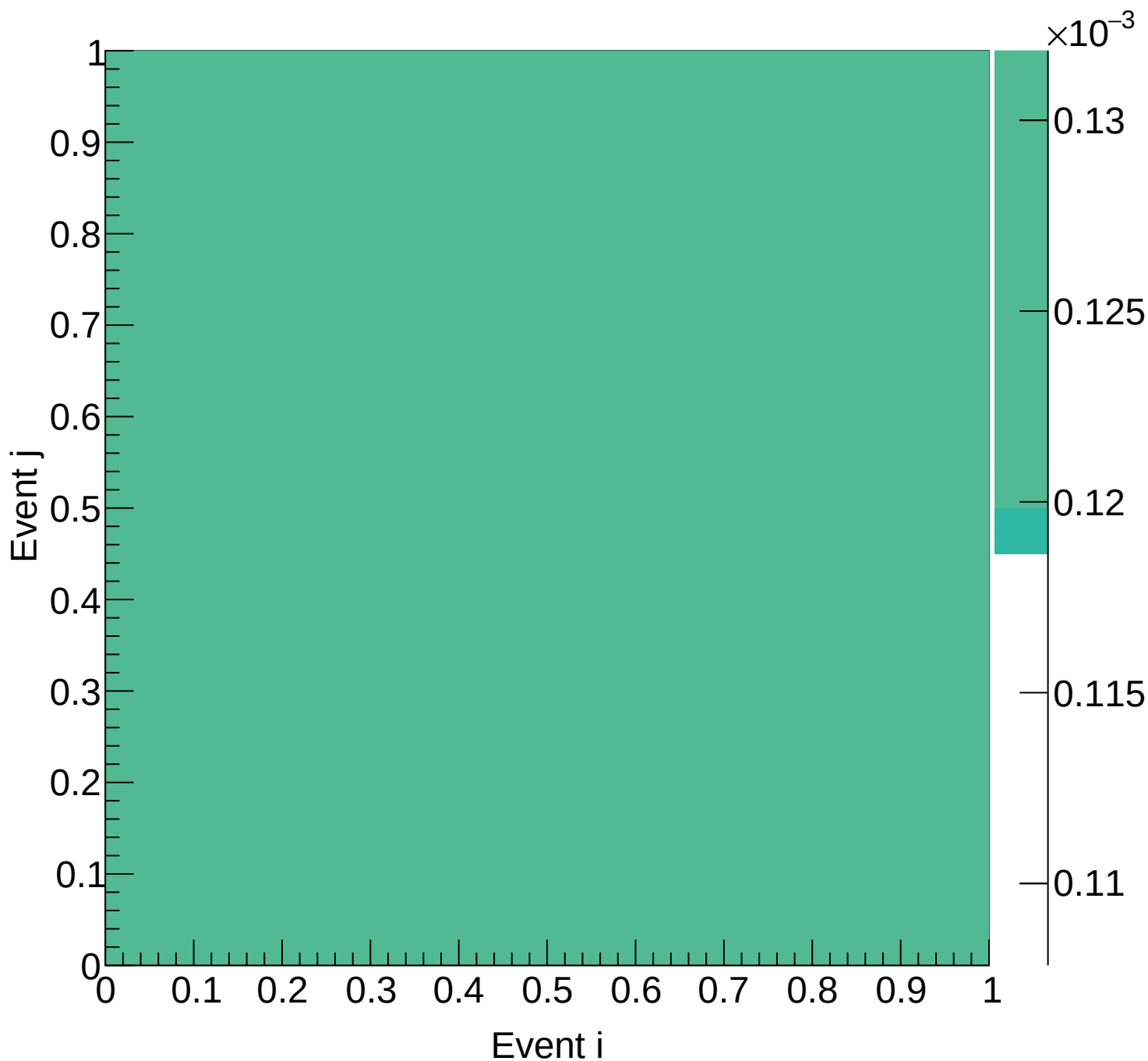
LH2 (mix) Covariance | M: [4.8, 5.1) xF: [0.80, 0.85)
