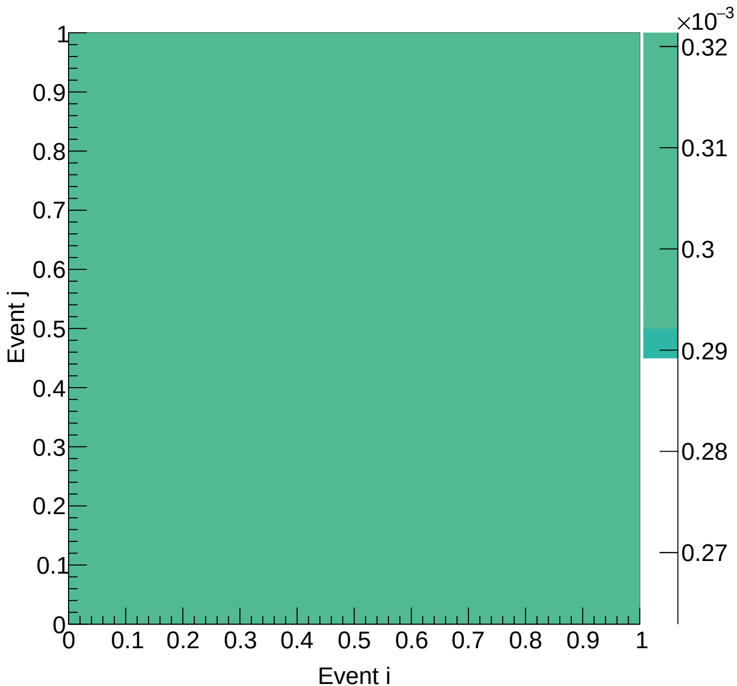
LH2 (mix) Covariance | M: [5.1, 5.4) xF: [0.80, 0.85)
