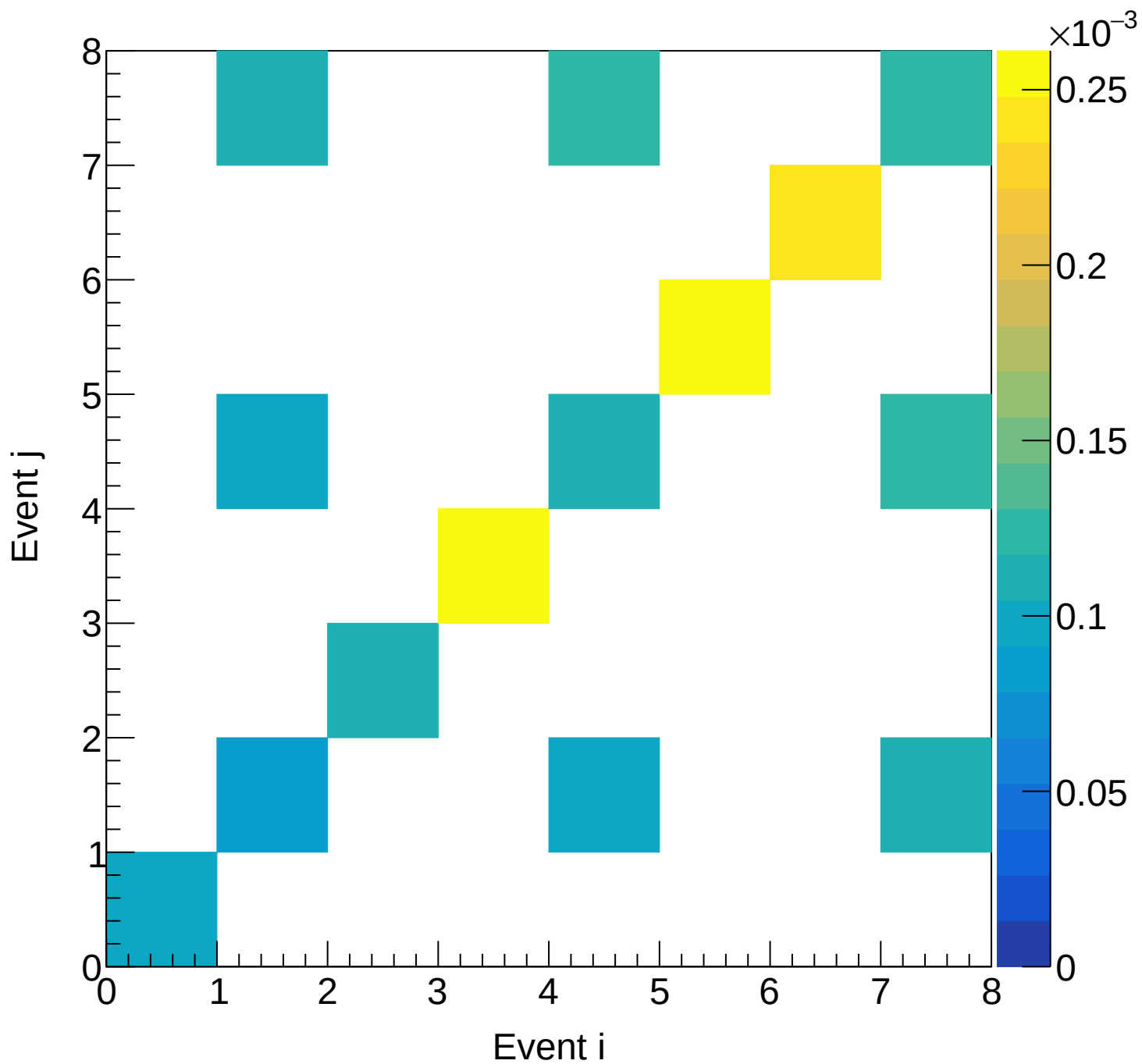
LH2 (mix) Covariance | M: [3.9, 4.2] xF: [0.85, 0.90)
