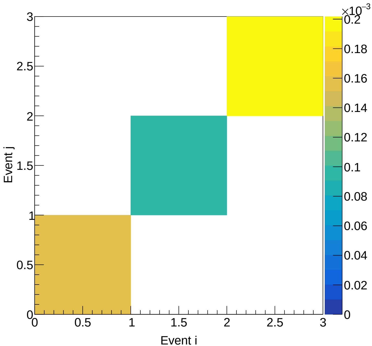
LH2 (mix) Covariance | M: [4.2, 4.5) xF: [0.85, 0.90)
