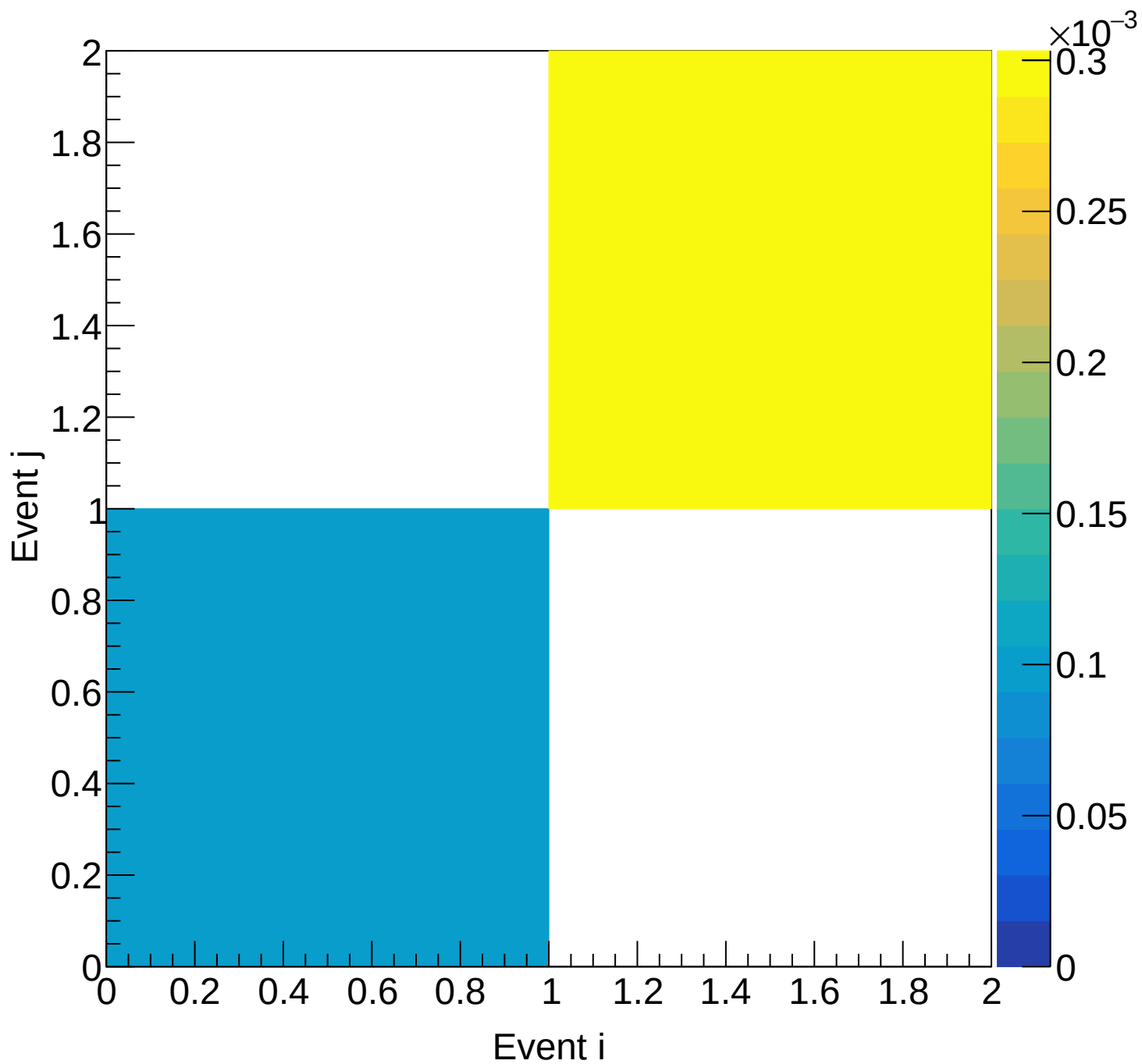
LH2 (mix) Covariance | M: [4.5, 4.8) xF: [0.85, 0.90)
