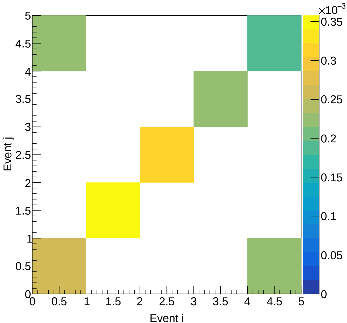
LH2 (mix) Covariance | M: [3.9, 4.2) xF: [0.90, 0.95)
