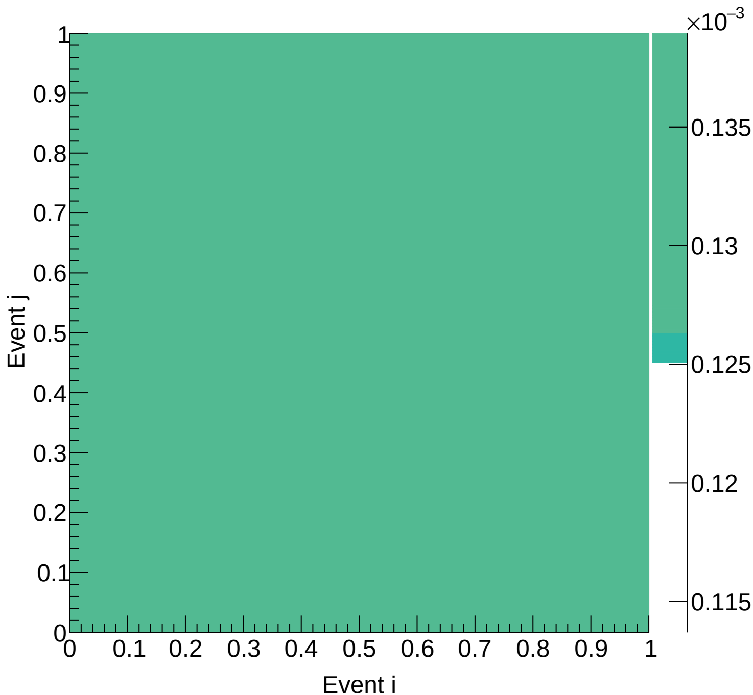
LH2 (mix) Covariance | M: [4.5, 4.8) xF: [0.90, 0.95)
