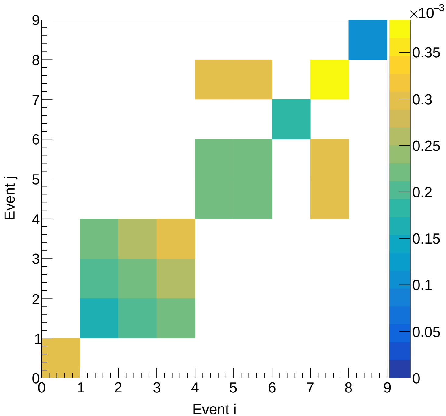
LH2 (mix) Covariance | M: [4.8, 5.1) xF: [0.00, 0.05)
