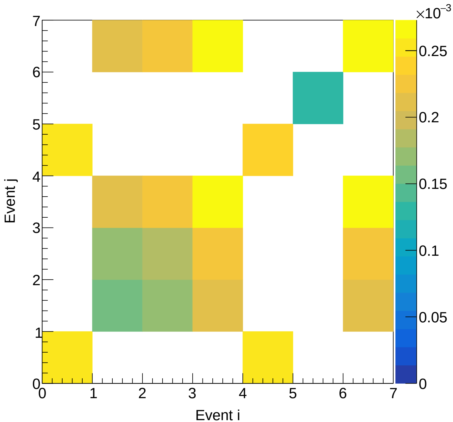
LH2 (mix) Covariance | M: [5.1, 5.4) xF: [0.00, 0.05)
