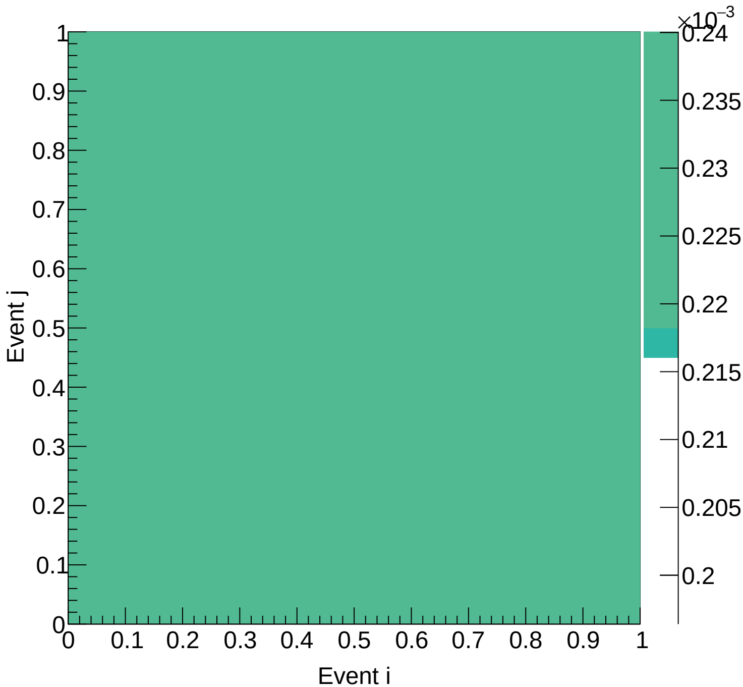
LH2 (mix) Covariance | M: [6.0, 6.3) xF: [0.00, 0.05)
