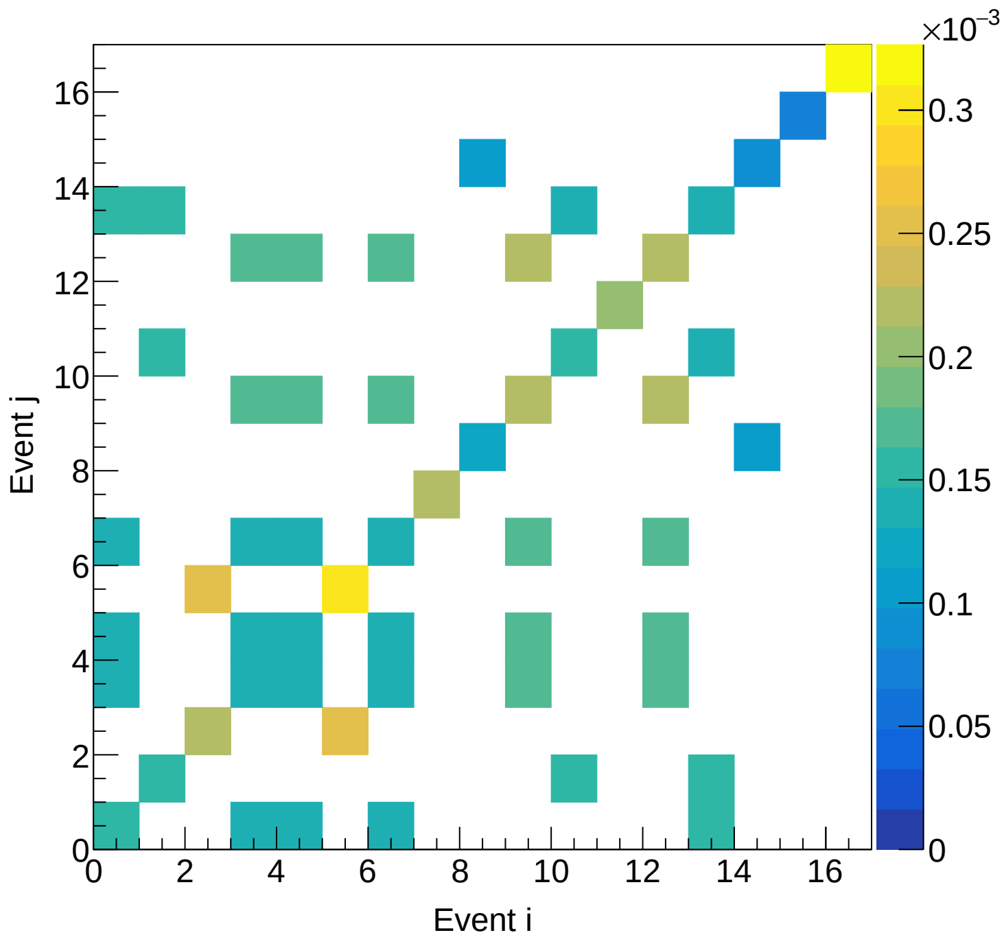
LH2 (mix) Covariance | M: [5.1, 5.4) xF: [0.05, 0.10)
