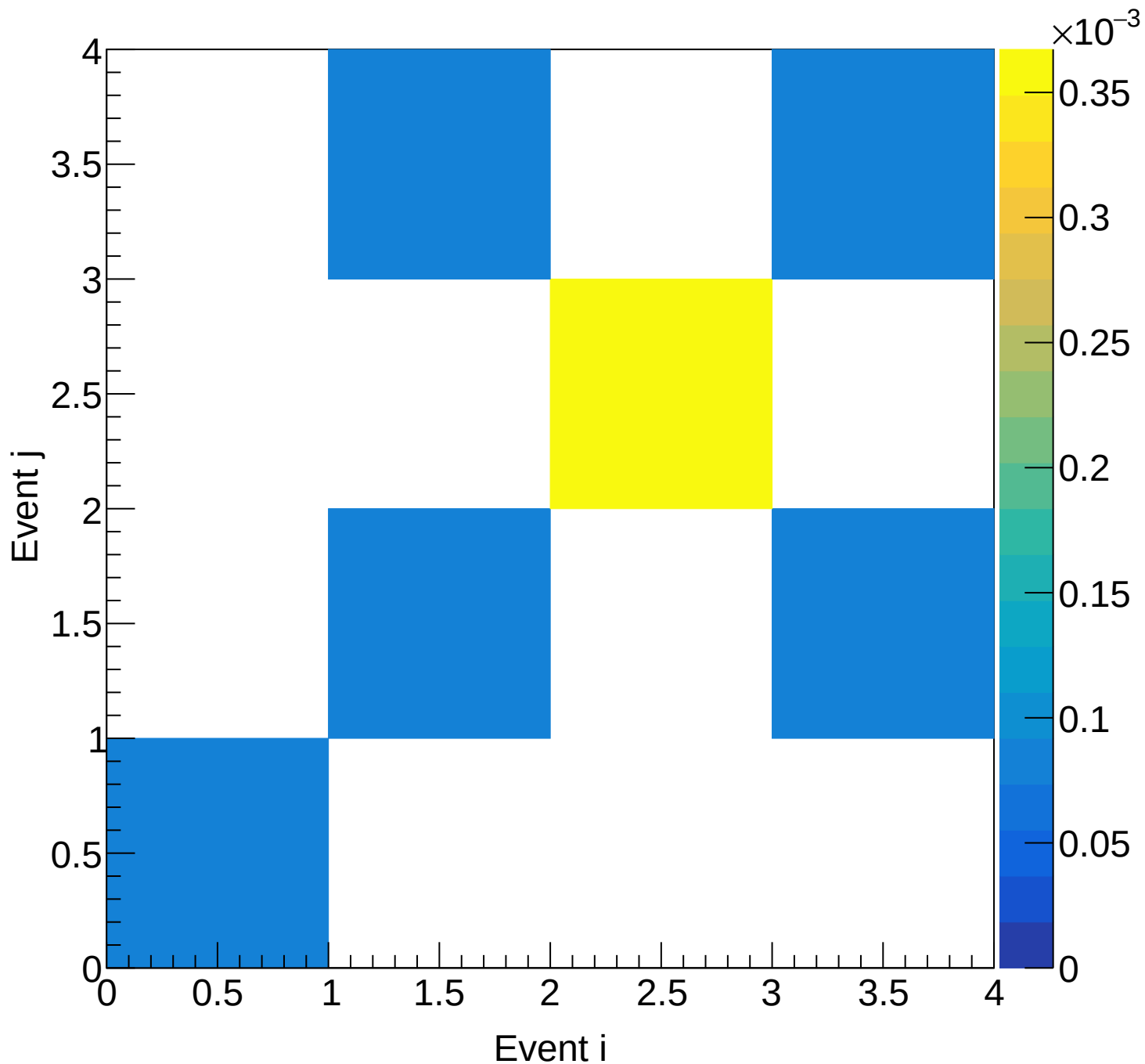
LH2 (mix) Covariance | M: [5.7, 6.0] xF: [0.05, 0.10)
