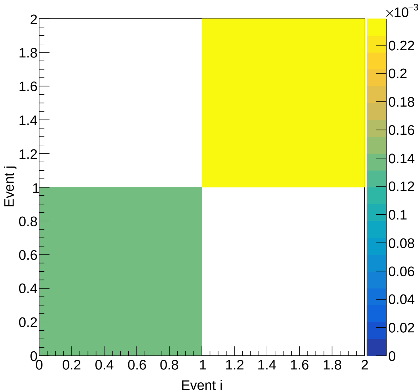
LH2 (mix) Covariance | M: [6.0, 6.3) xF: [0.05, 0.10)
