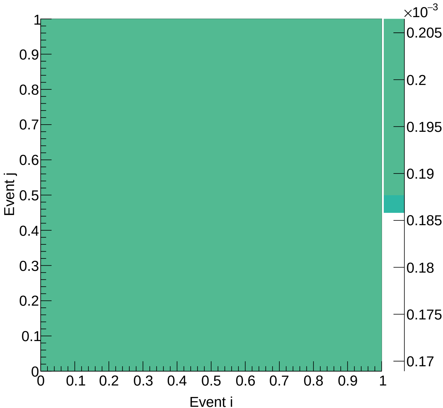
LH2 (mix) Covariance | M: [6.9, 7.5) xF: [0.10, 0.15)
