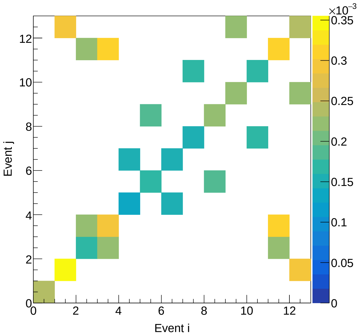
LH2 (mix) Covariance | M: [5.1, 5.4) xF: [0.10, 0.15)
