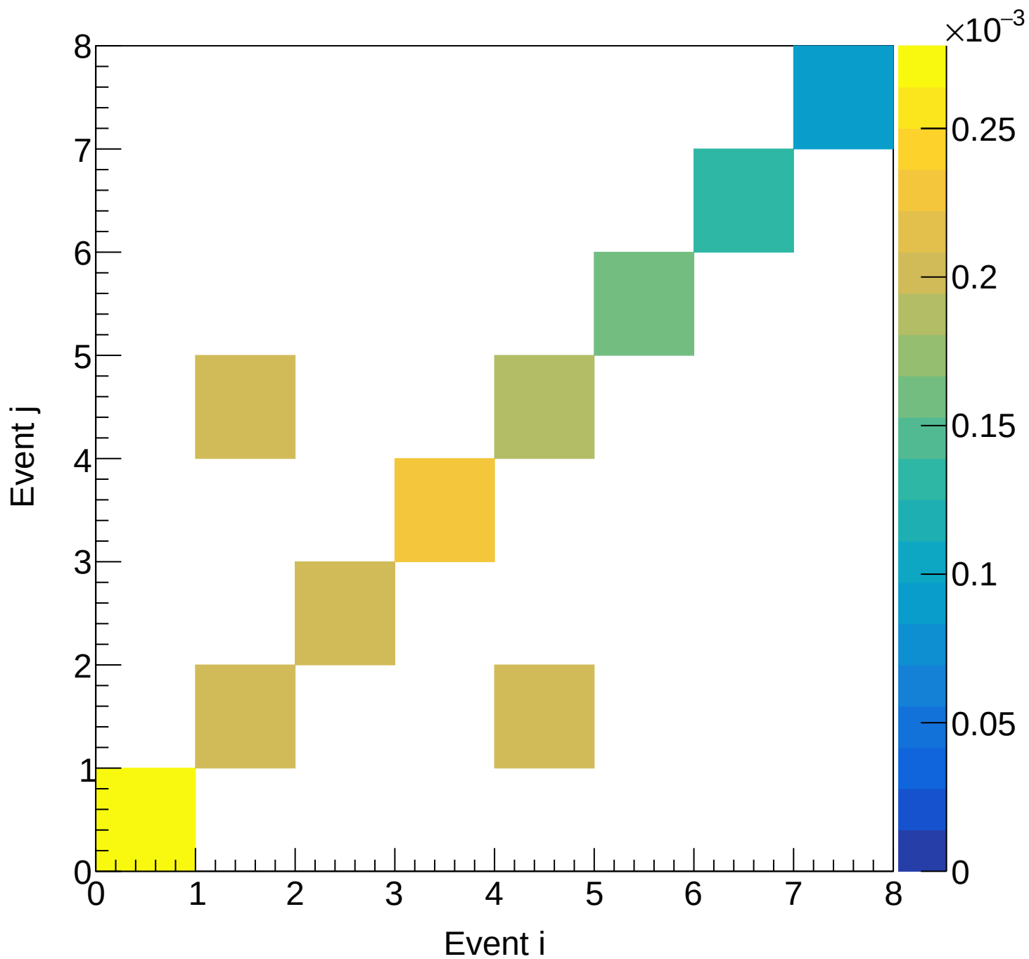
LH2 (mix) Covariance | M: [5.4, 5.7) xF: [0.10, 0.15)
