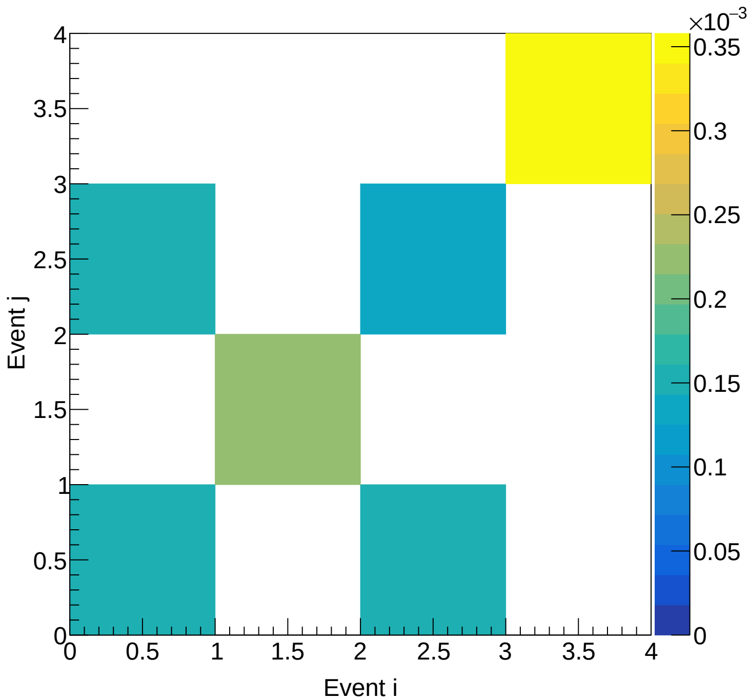
LH2 (mix) Covariance | M: [6.0, 6.3) xF: [0.10, 0.15)
