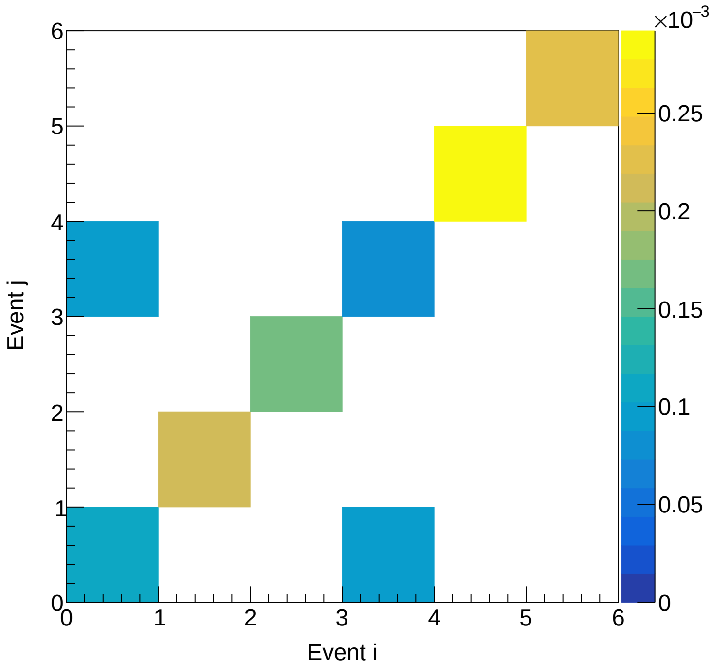
LH2 (mix) Covariance | M: [3.9, 4.2) xF: [0.15, 0.20)
