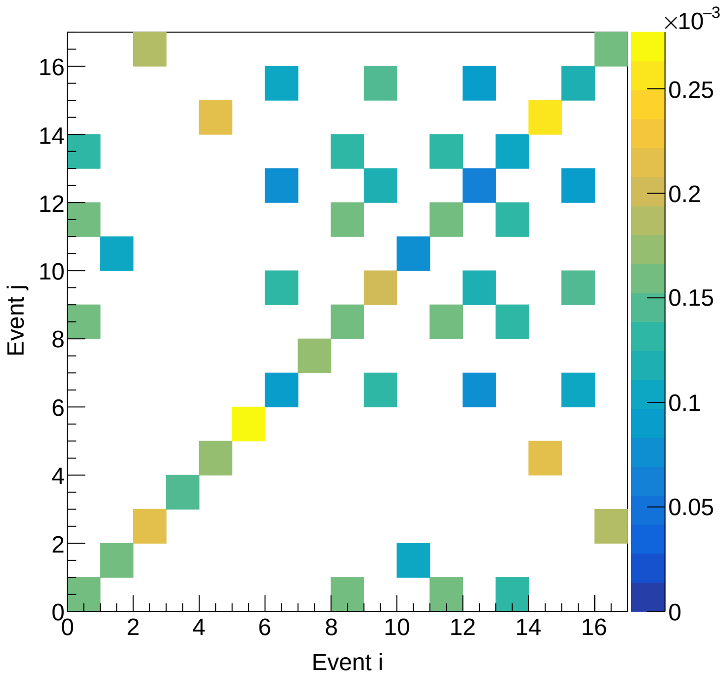
LH2 (mix) Covariance | M: [3.9, 4.2) xF: [0.20, 0.25)
