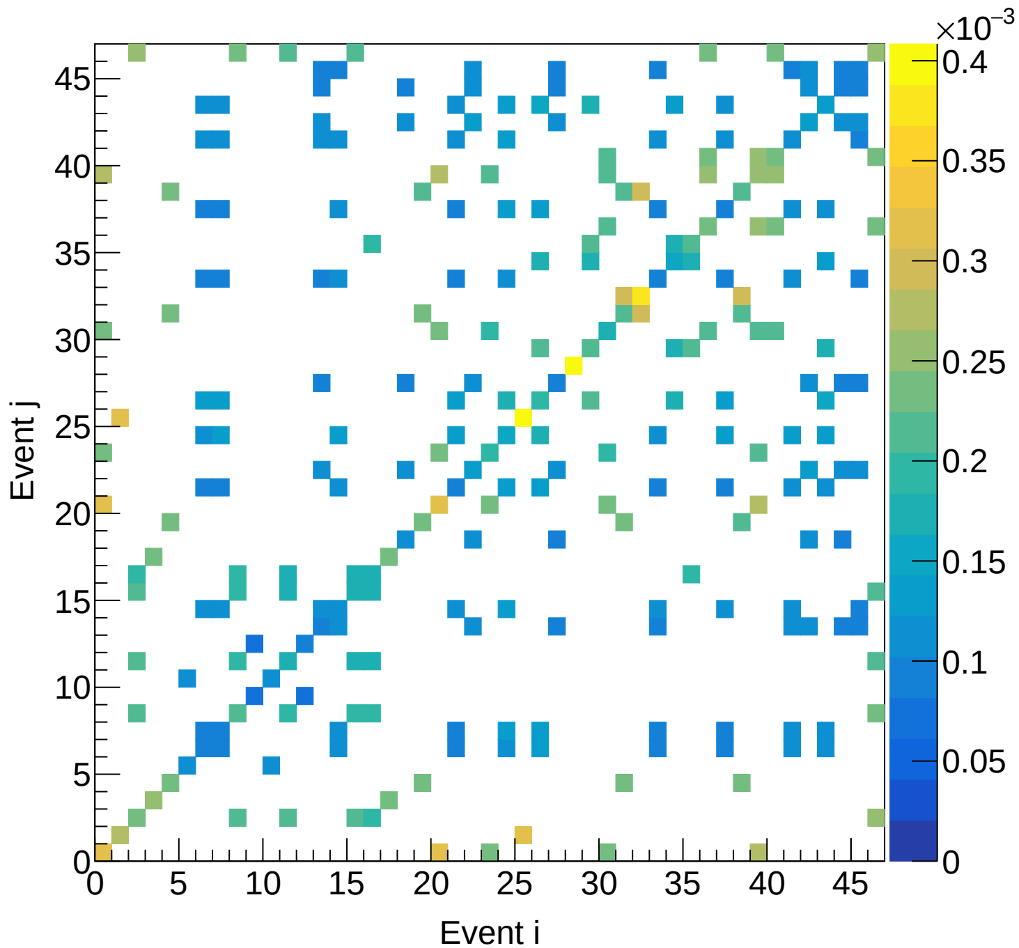
LH2 (mix) Covariance | M: [4.2, 4.5) xF: [0.20, 0.25)
