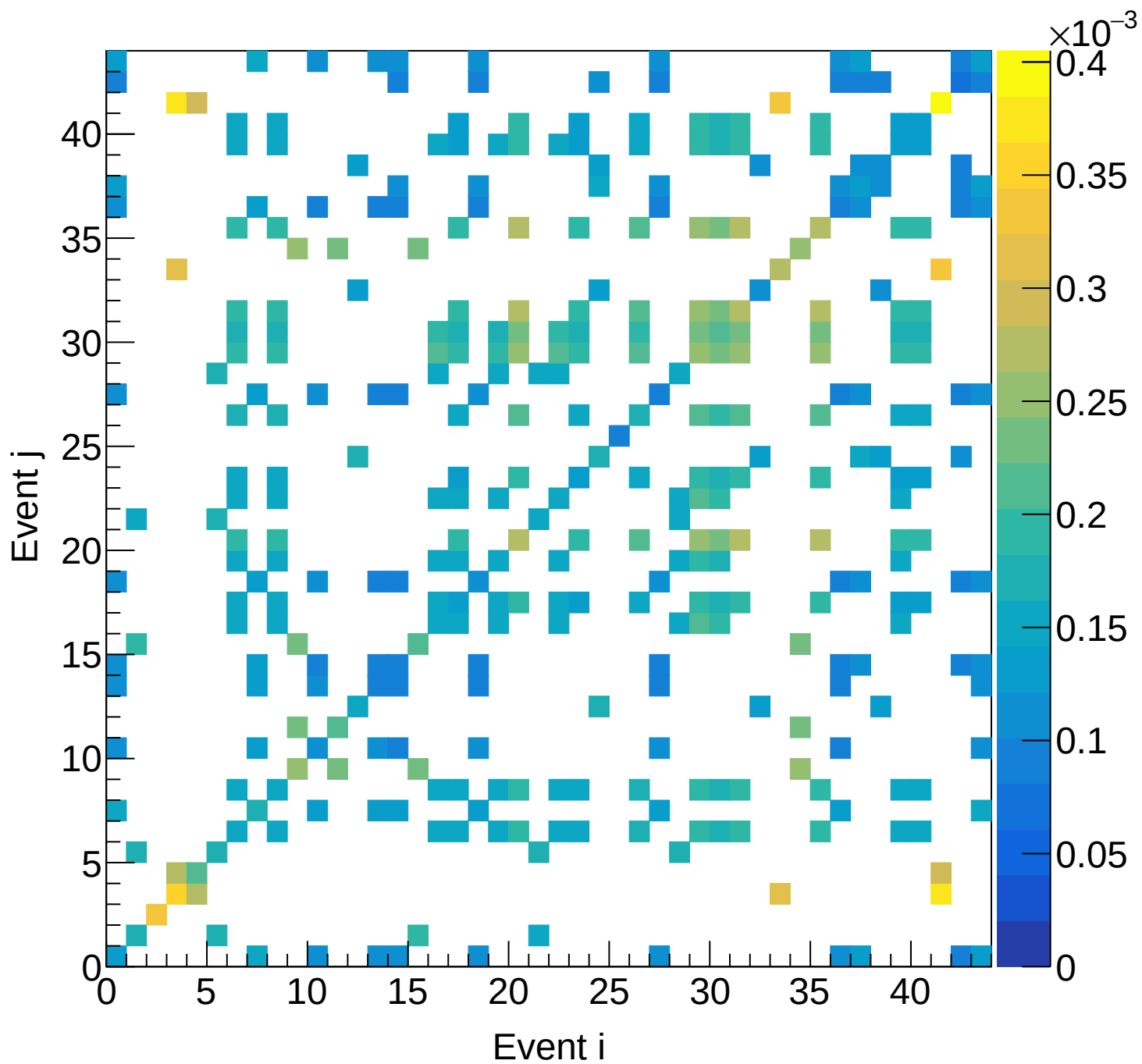
LH2 (mix) Covariance | M: [4.5, 4.8) xF: [0.20, 0.25)
