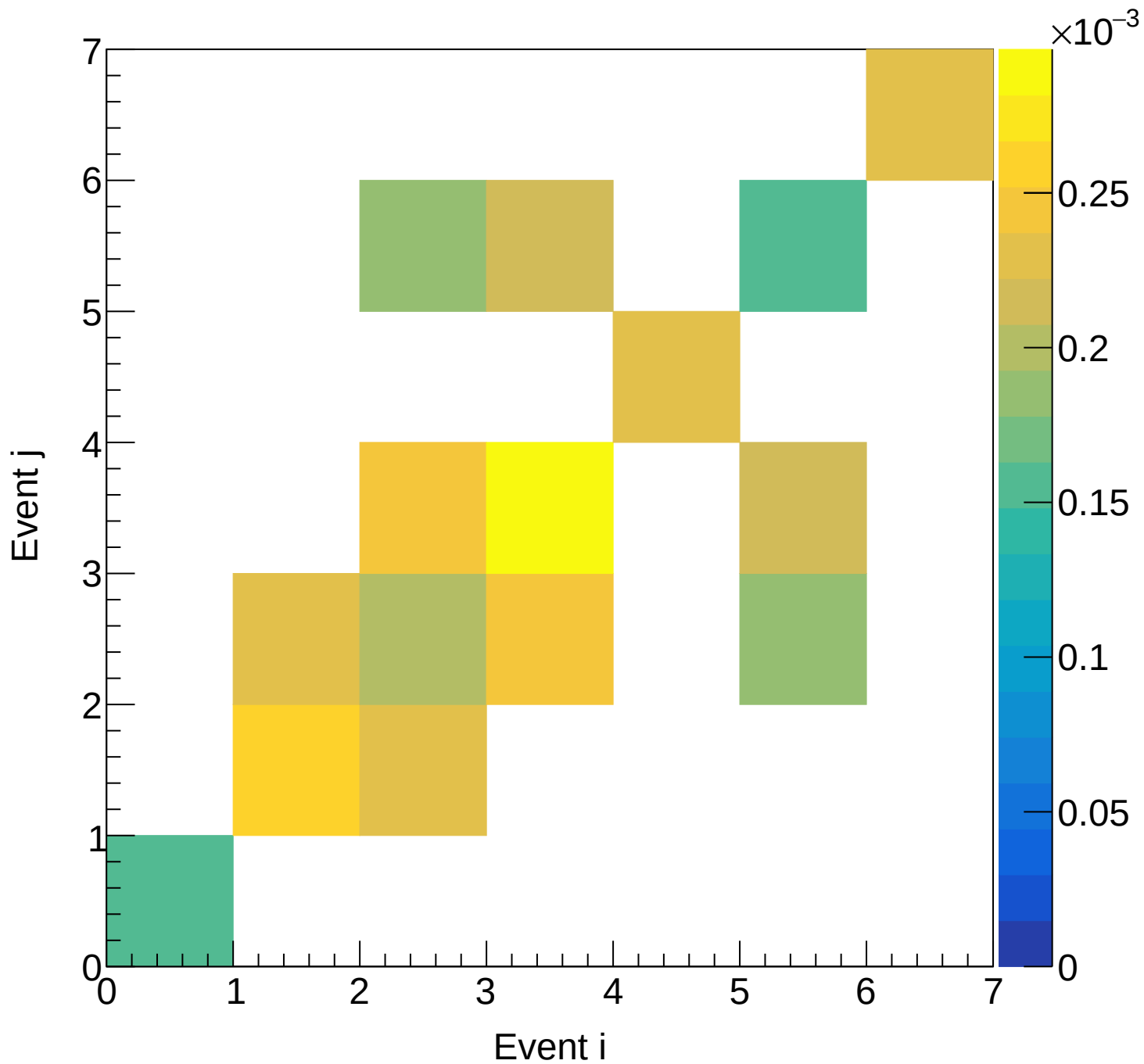
LH2 (mix) Covariance | M: [5.7, 6.0) xF: [0.20, 0.25)
