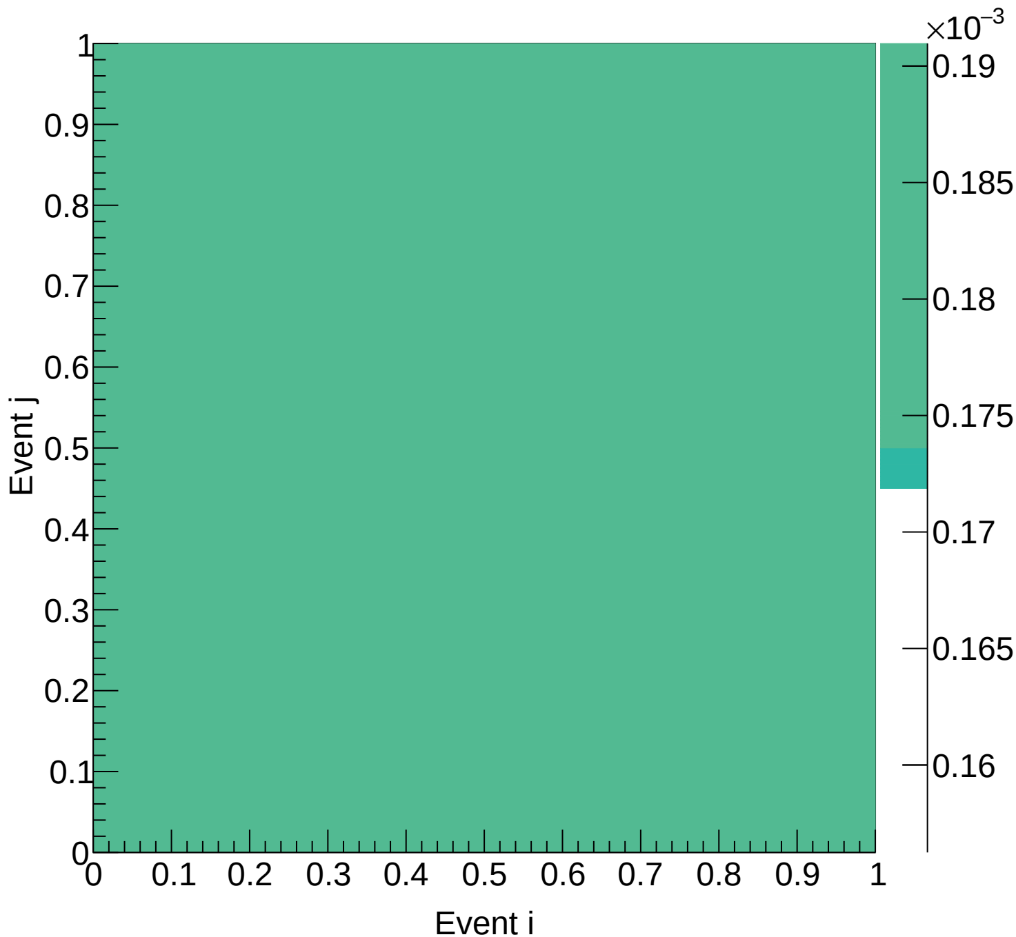
LH2 (mix) Covariance | M: [6.6, 6.9) xF: [0.20, 0.25)
