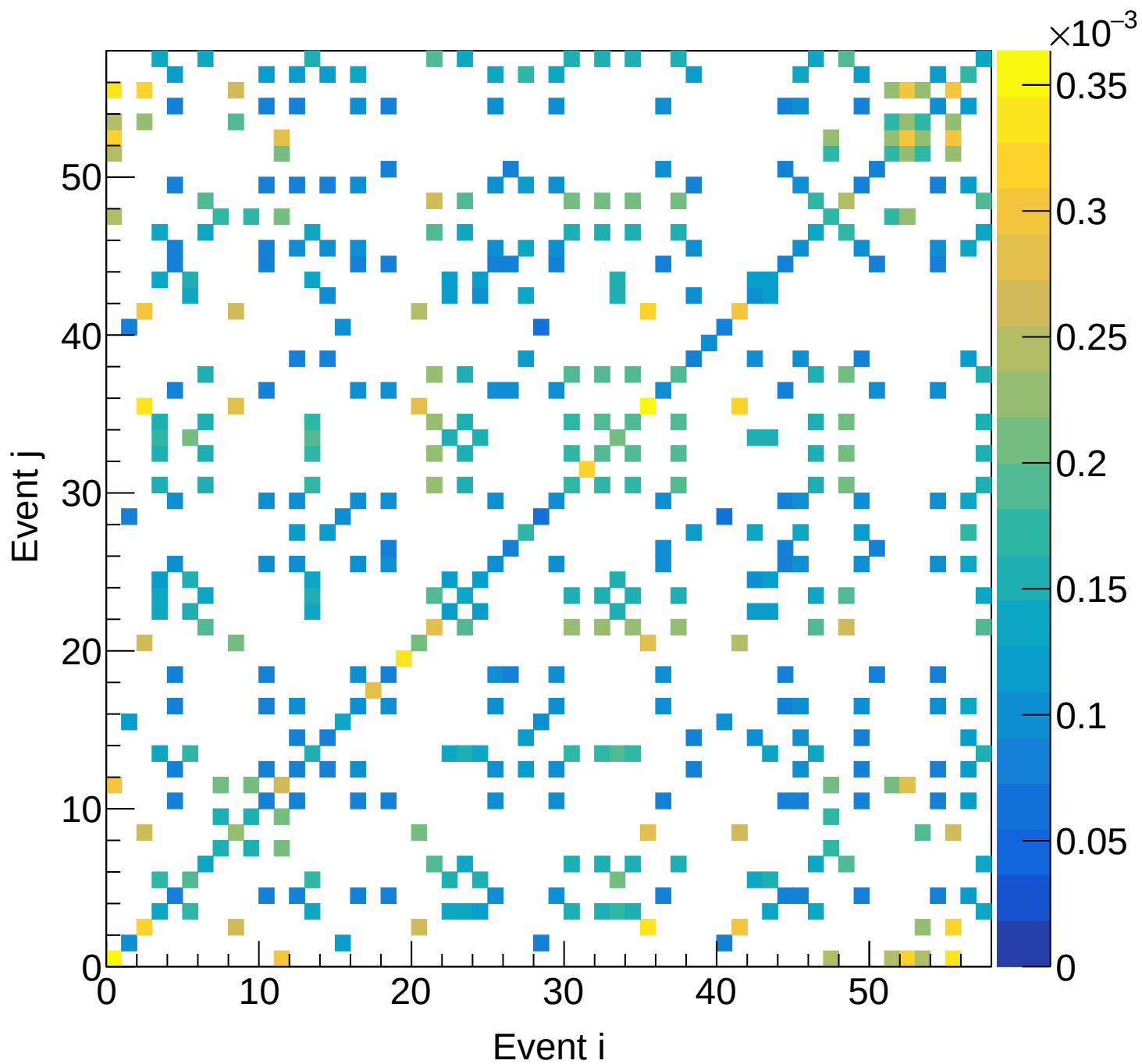
LH2 (mix) Covariance | M: [4.2, 4.5) xF: [0.25, 0.30)
