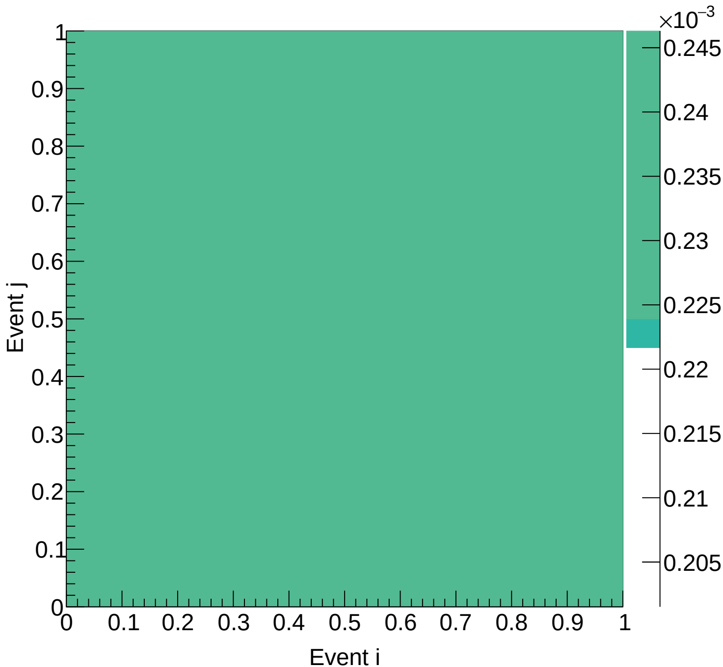
LH2 (mix) Covariance | M: [6.9, 7.5) xF: [0.25, 0.30)
