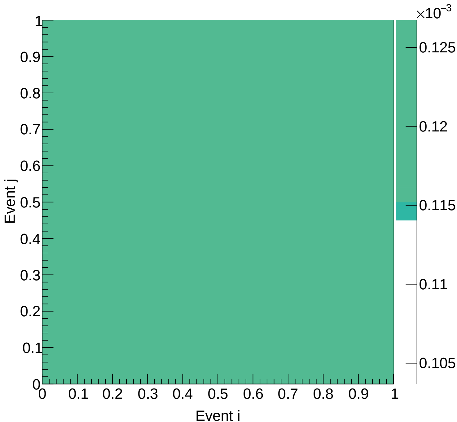
LH2 (mix) Covariance | M: [6.6, 6.9) xF: [0.25, 0.30)
