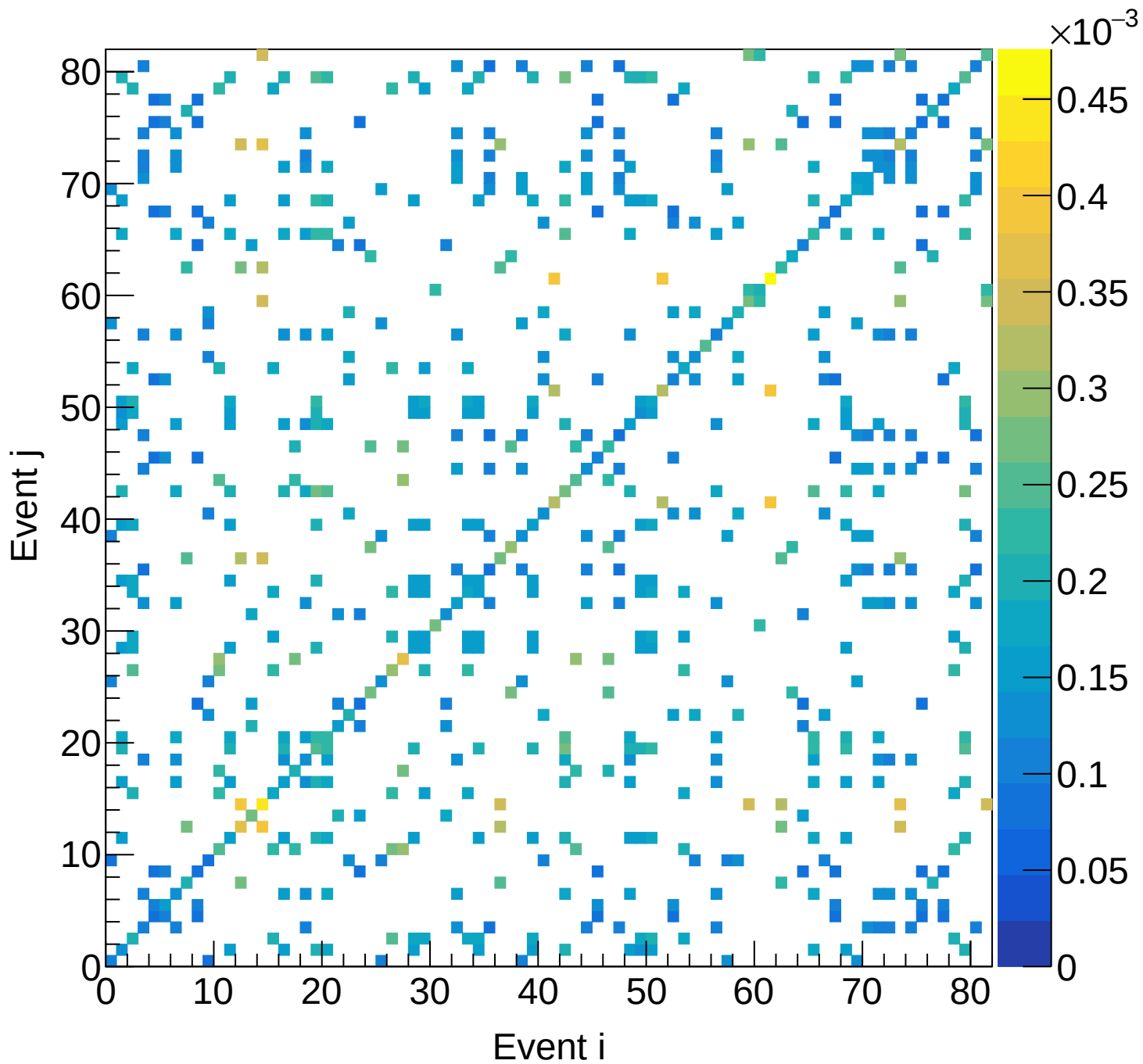
LH2 (mix) Covariance | M: [3.9, 4.2) xF: [0.30, 0.35)
