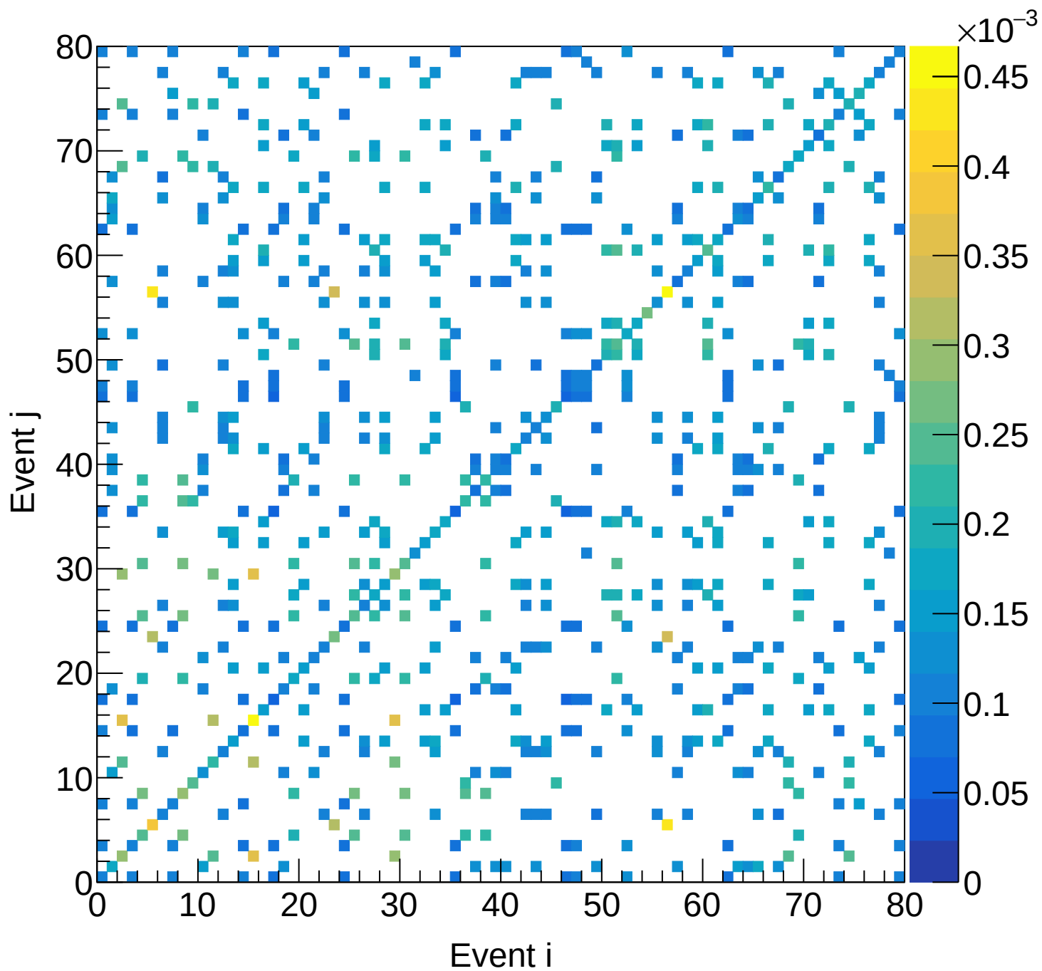
LH2 (mix) Covariance | M: [4.2, 4.5) xF: [0.30, 0.35)
