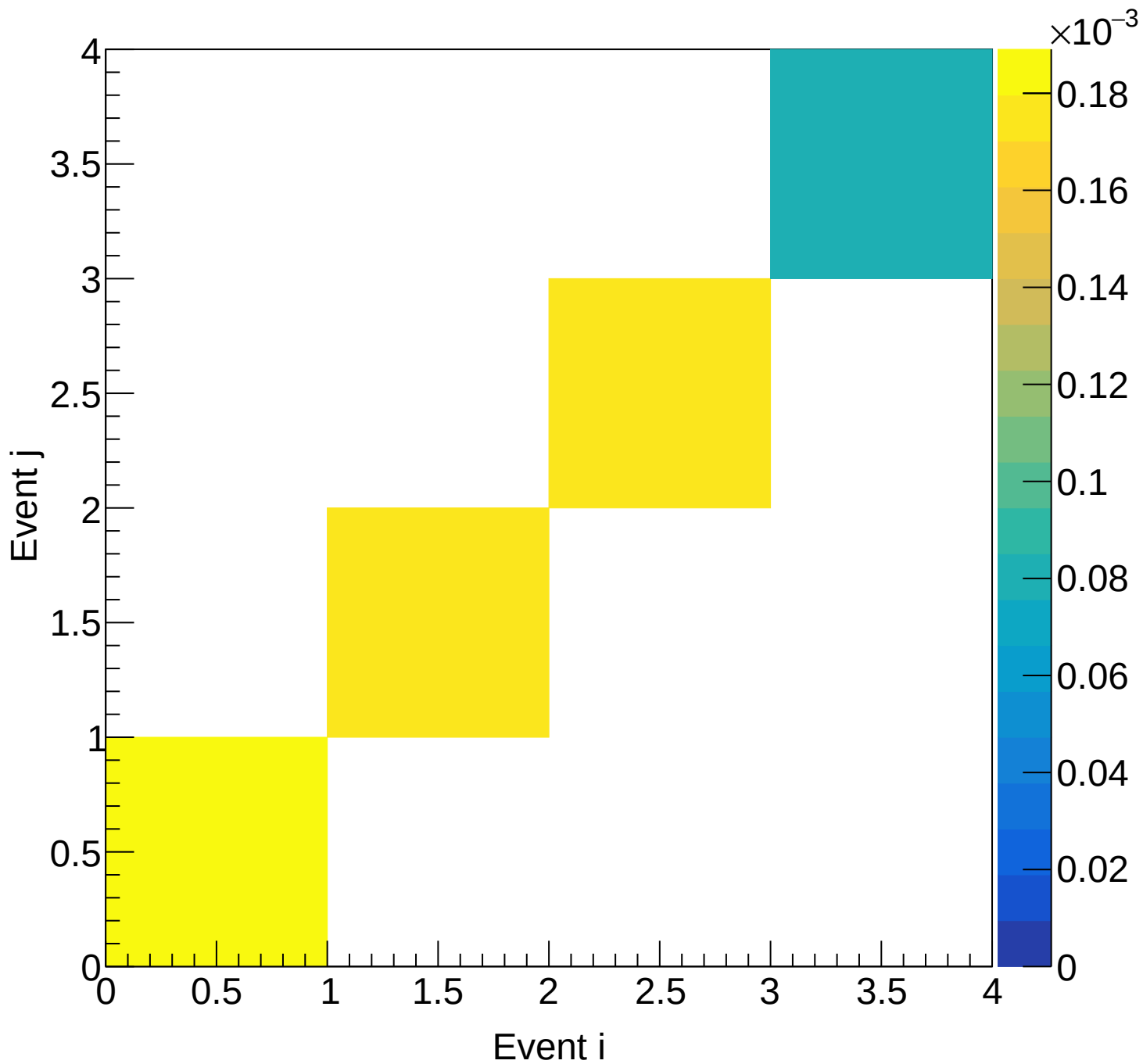
LH2 (mix) Covariance | M: [5.7, 6.0] xF: [0.30, 0.35)
