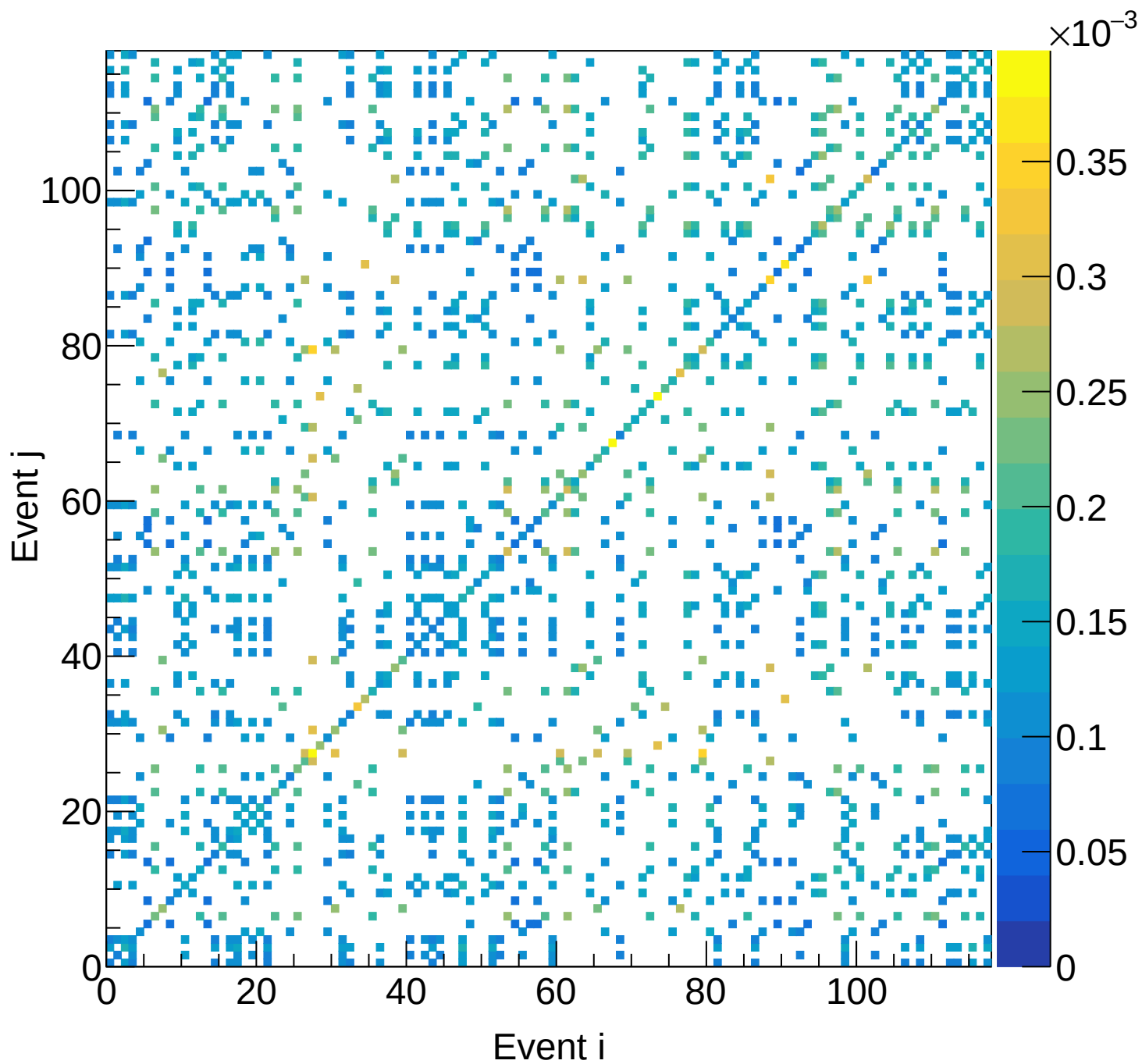
LH2 (mix) Covariance | M: [3.9, 4.2) xF: [0.35, 0.40)
