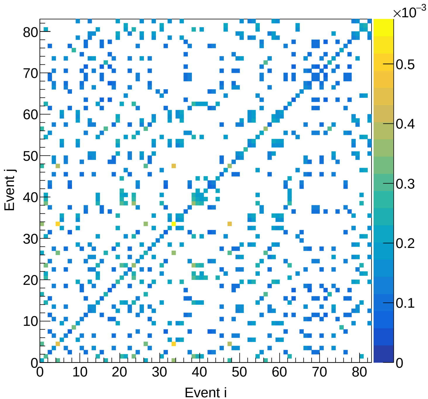
LH2 (mix) Covariance | M: [4.2, 4.5) xF: [0.35, 0.40)
