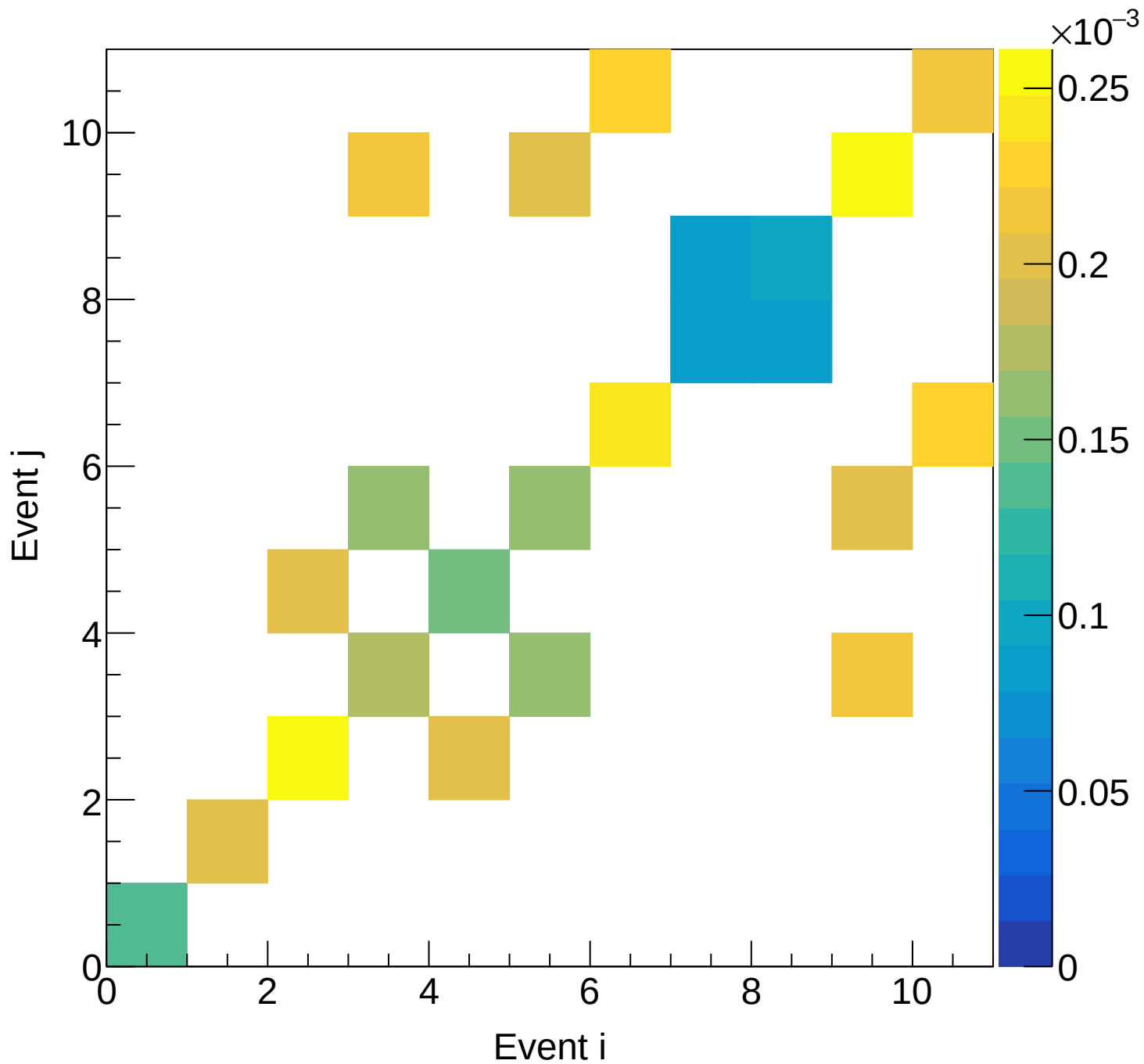
LH2 (mix) Covariance | M: [5.1, 5.4) xF: [0.35, 0.40)
