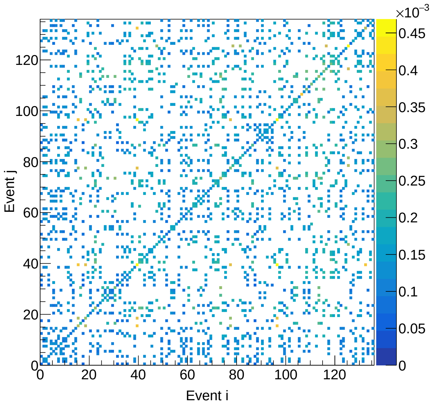
LH2 (mix) Covariance | M: [3.9, 4.2) xF: [0.40, 0.45)
