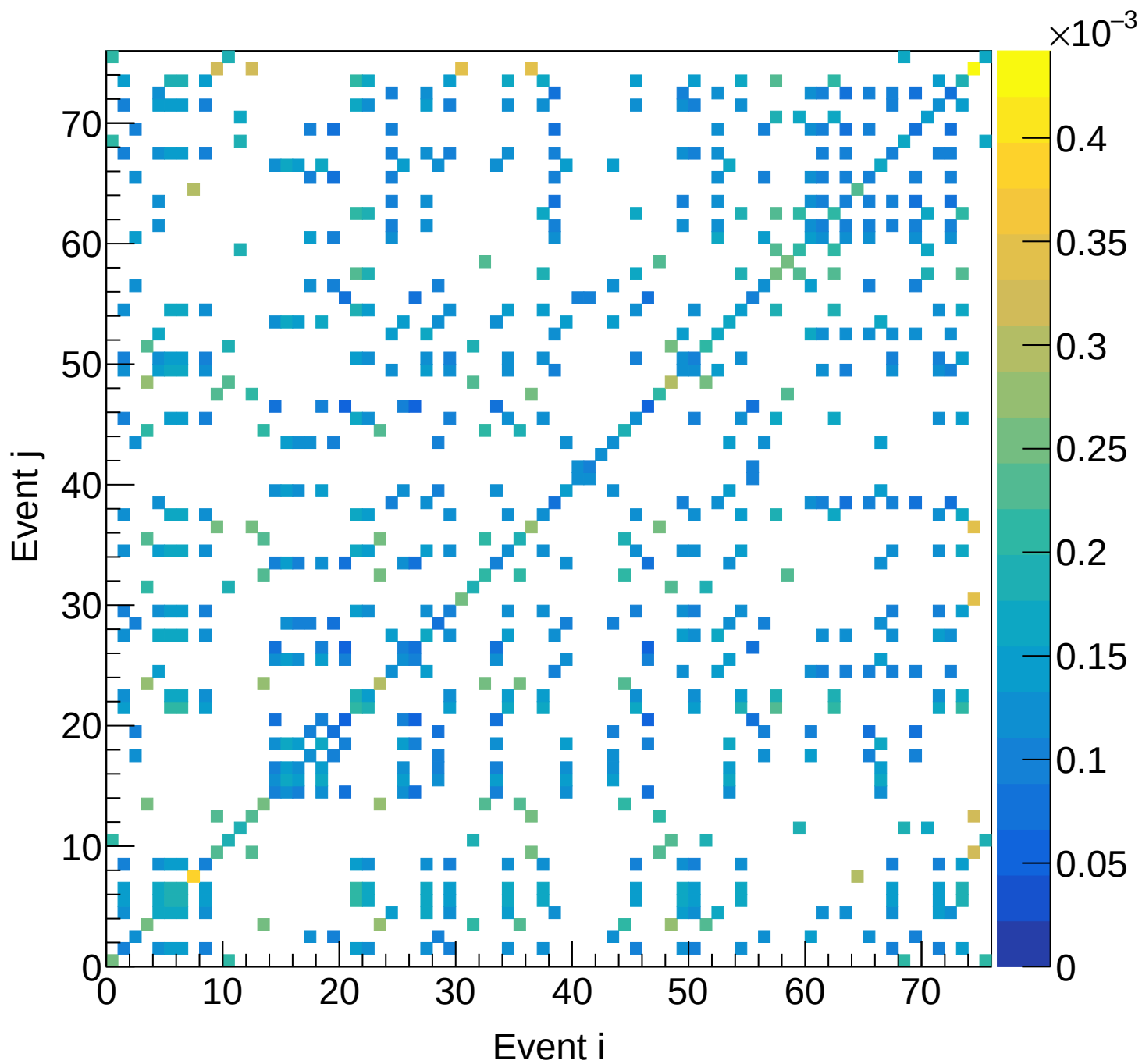
LH2 (mix) Covariance | M: [4.2, 4.5) xF: [0.40, 0.45)
