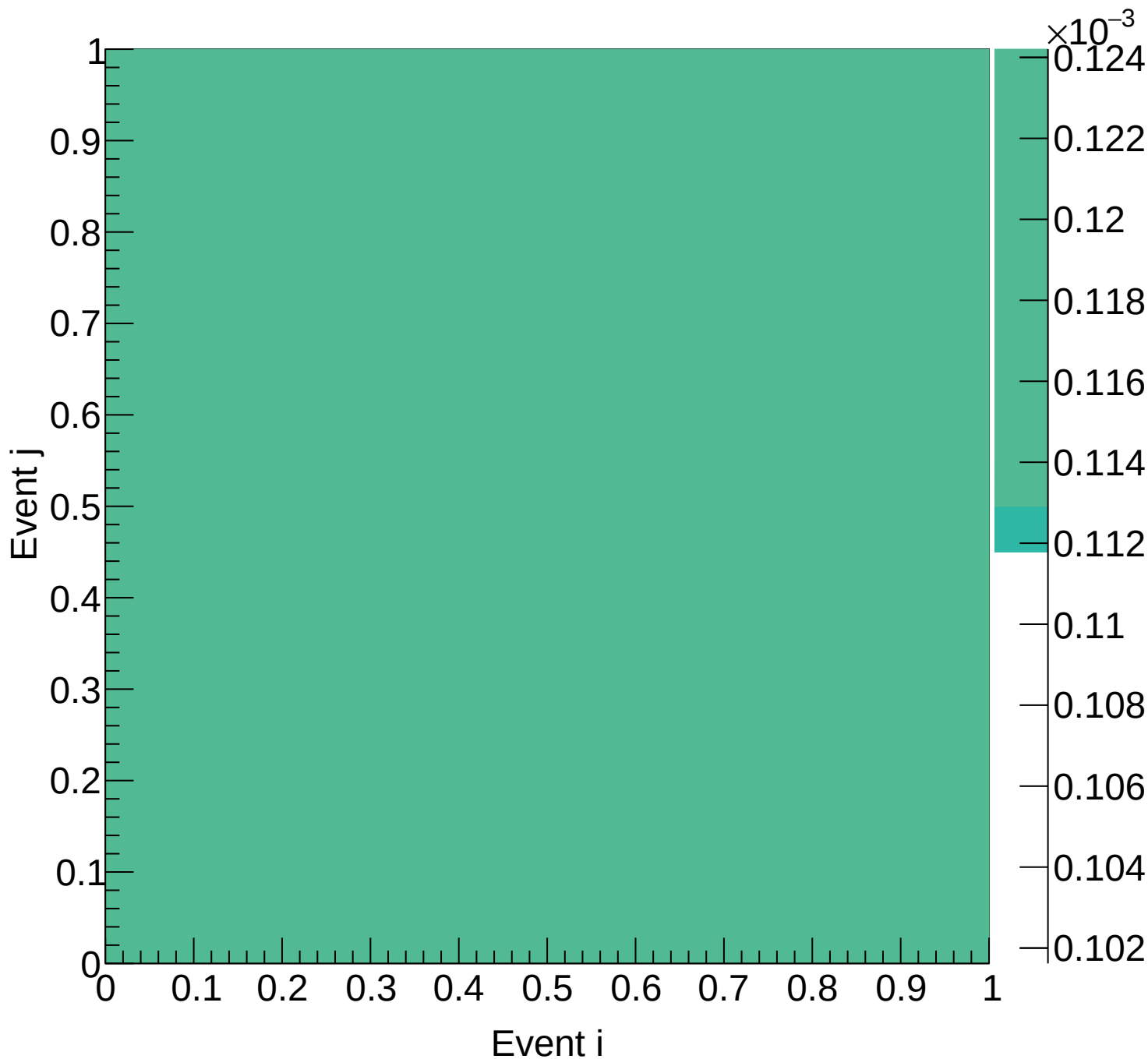
LH2 (mix) Covariance | M: [6.9, 7.5] xF: [0.40, 0.45)
