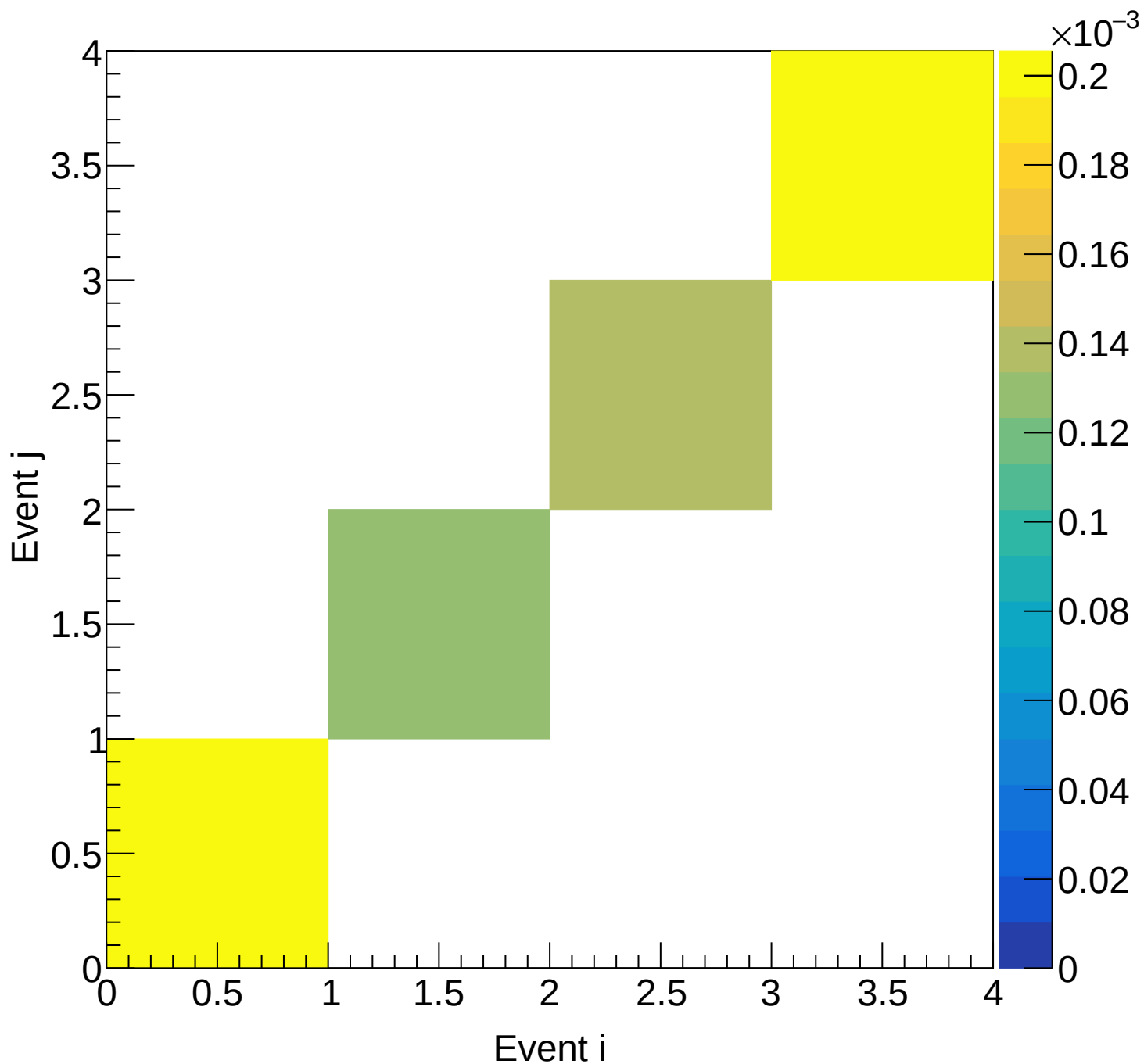
LH2 (mix) Covariance | M: [5.4, 5.7) xF: [0.40, 0.45)
