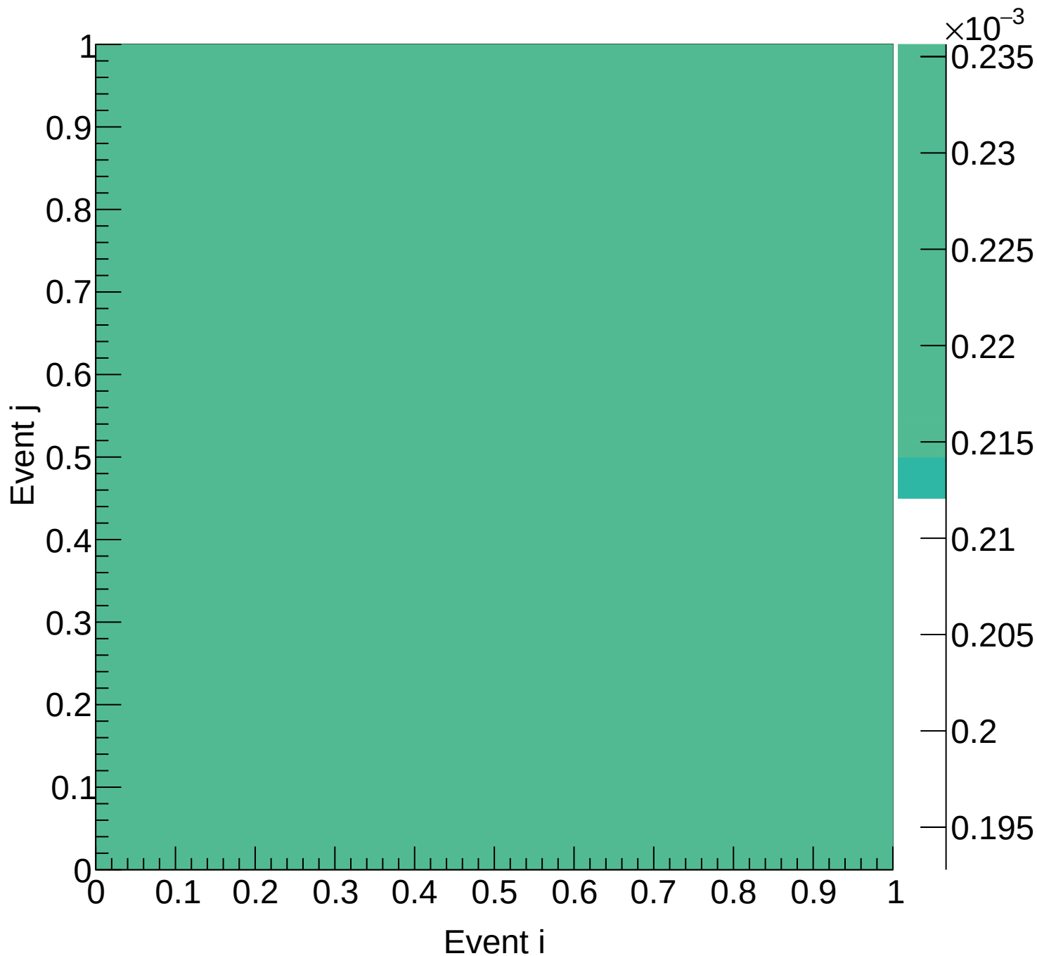
LH2 (mix) Covariance | M: [6.0, 6.3) xF: [0.40, 0.45)
