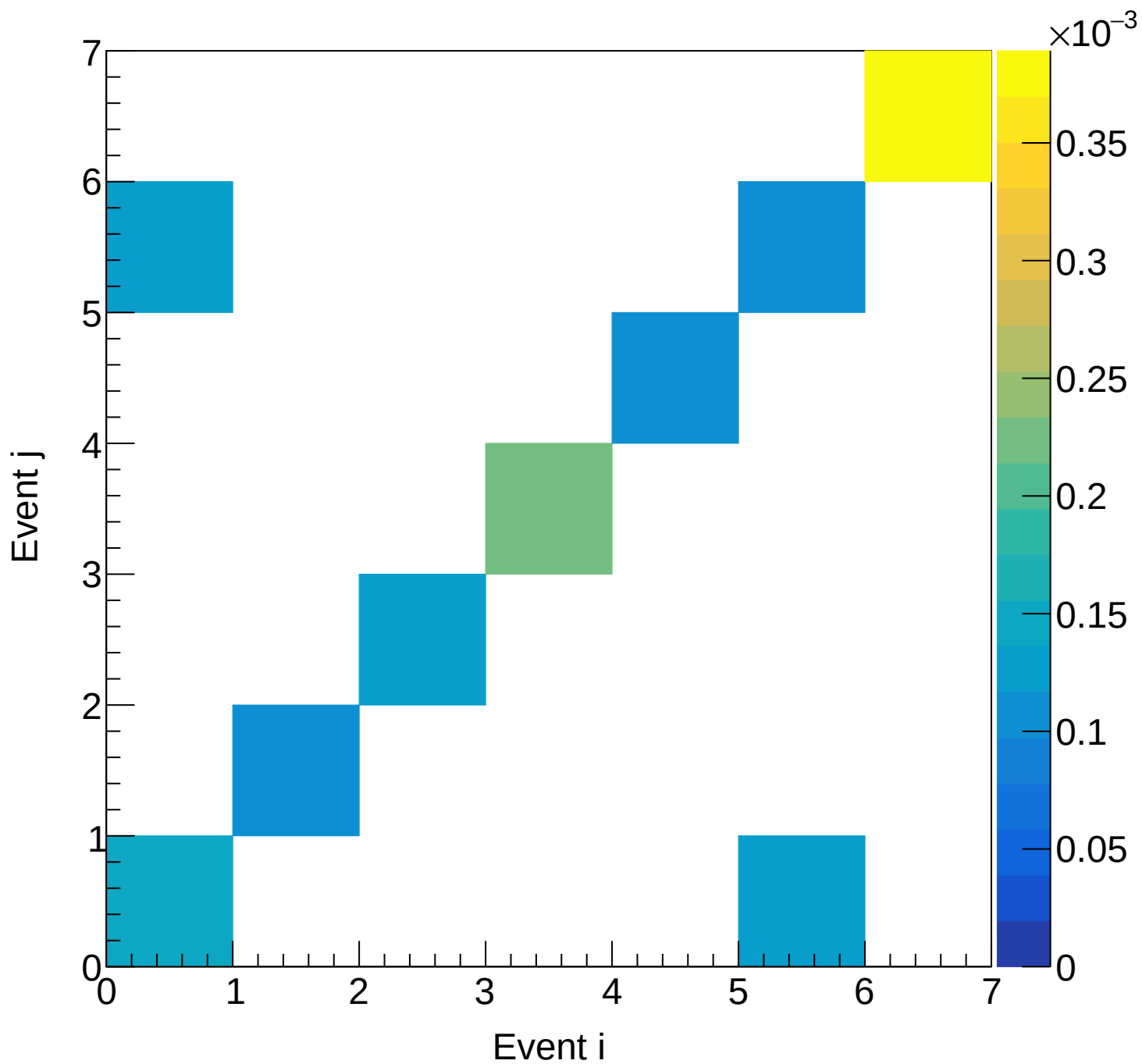
LH2 (total) Covariance | M: [6.9, 7.5) xF: [-0.05, 0.00)
