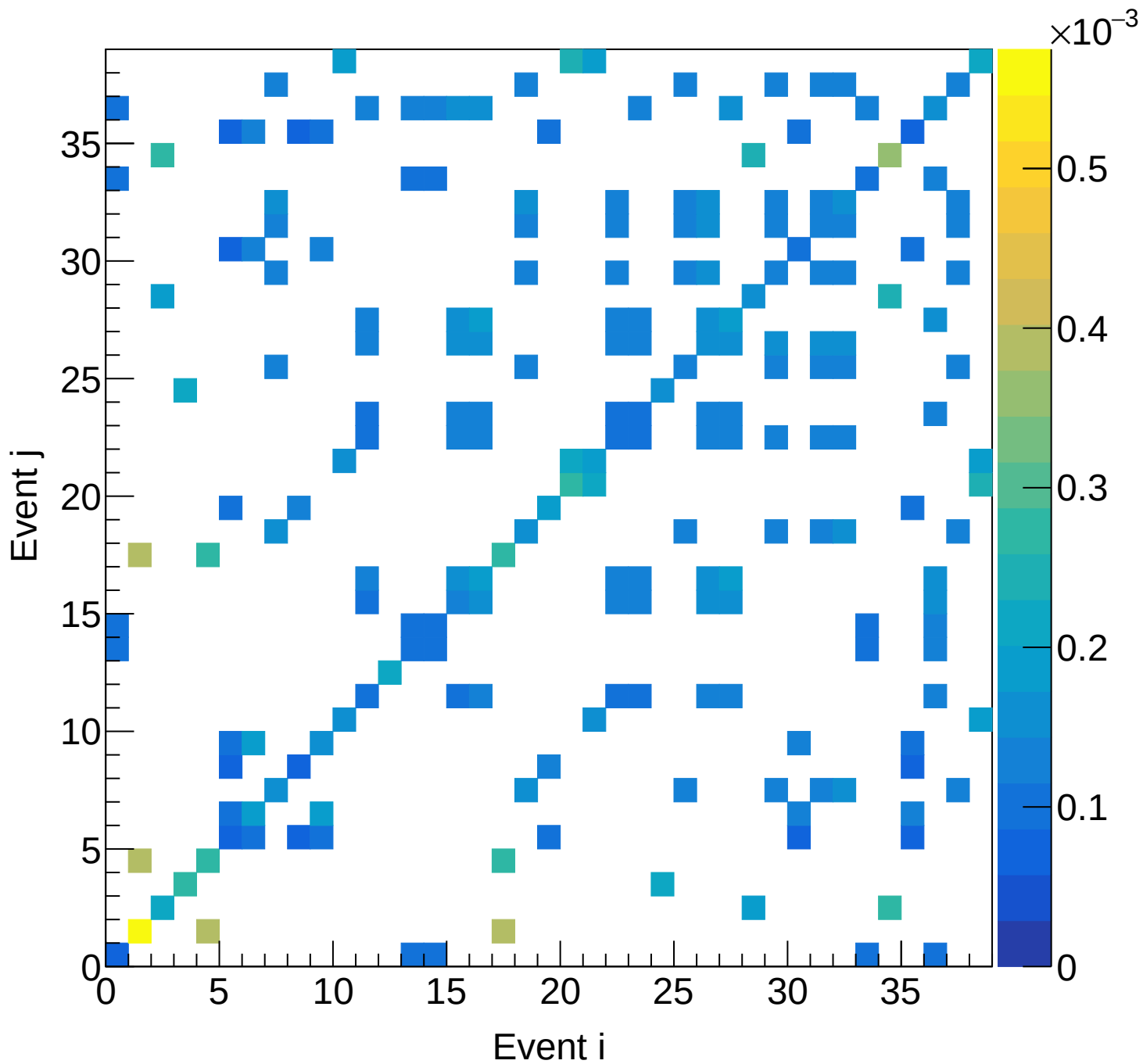
LH2 (total) Covariance | M: [5.7, 6.0] xF: [-0.05, 0.00]
