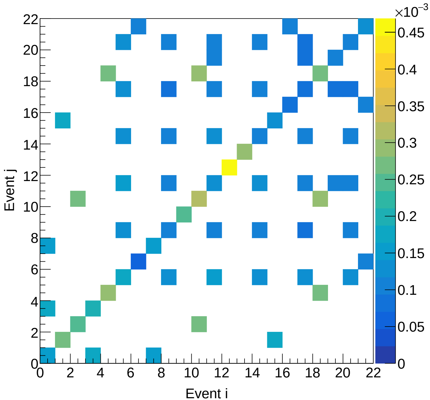
LH2 (total) Covariance | M: [6.0, 6.3) xF: [-0.05, 0.00)
