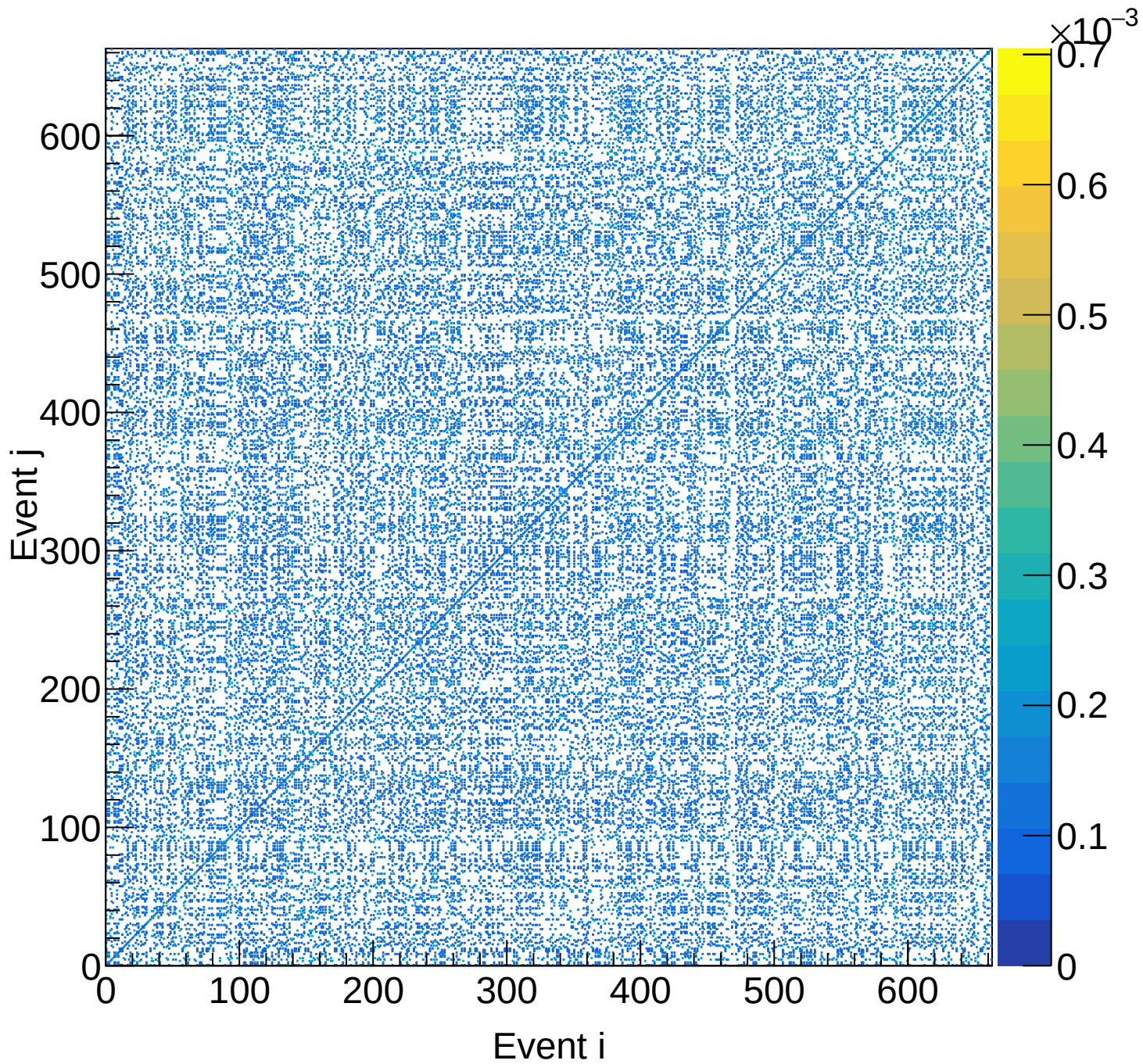
LH2 (total) Covariance | M: [4.2, 4.5) xF: [0.45, 0.50)
