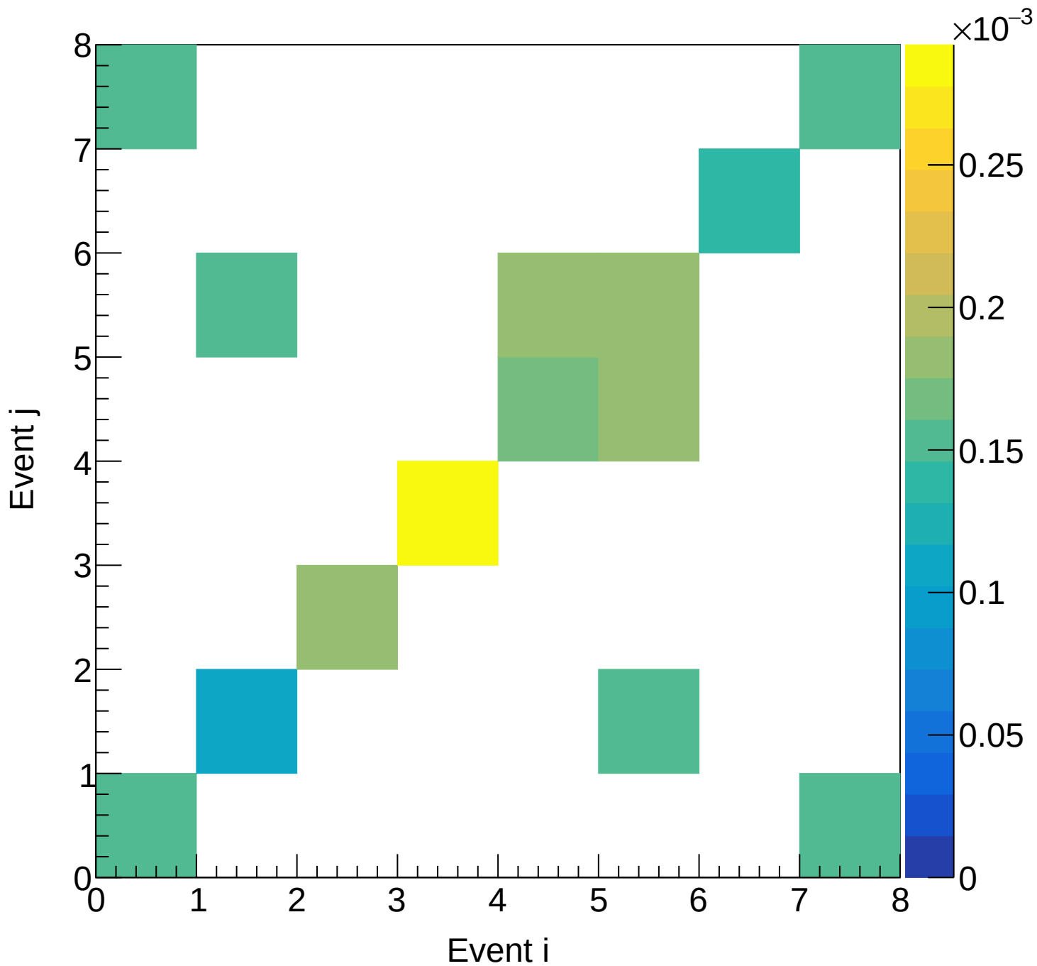
LH2 (total) Covariance | M: [7.5, 8.8) xF: [0.45, 0.50)
