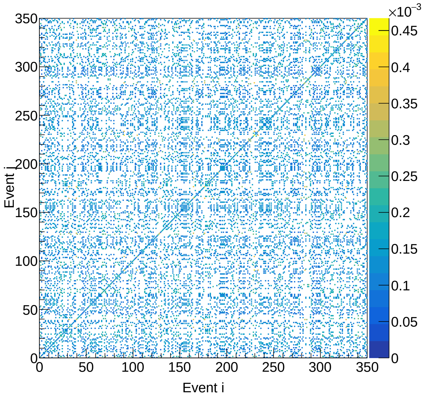
LH2 (total) Covariance | M: [4.8, 5.1) xF: [0.45, 0.50)
