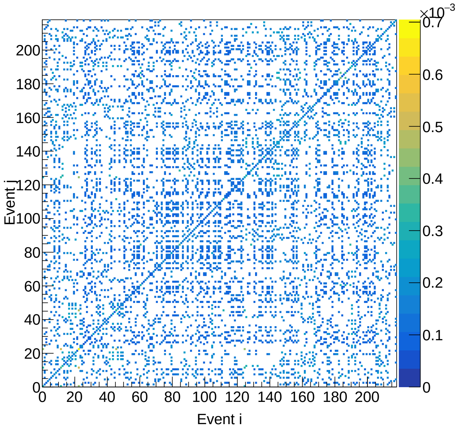
LH2 (total) Covariance | M: [5.1, 5.4) xF: [0.45, 0.50)
