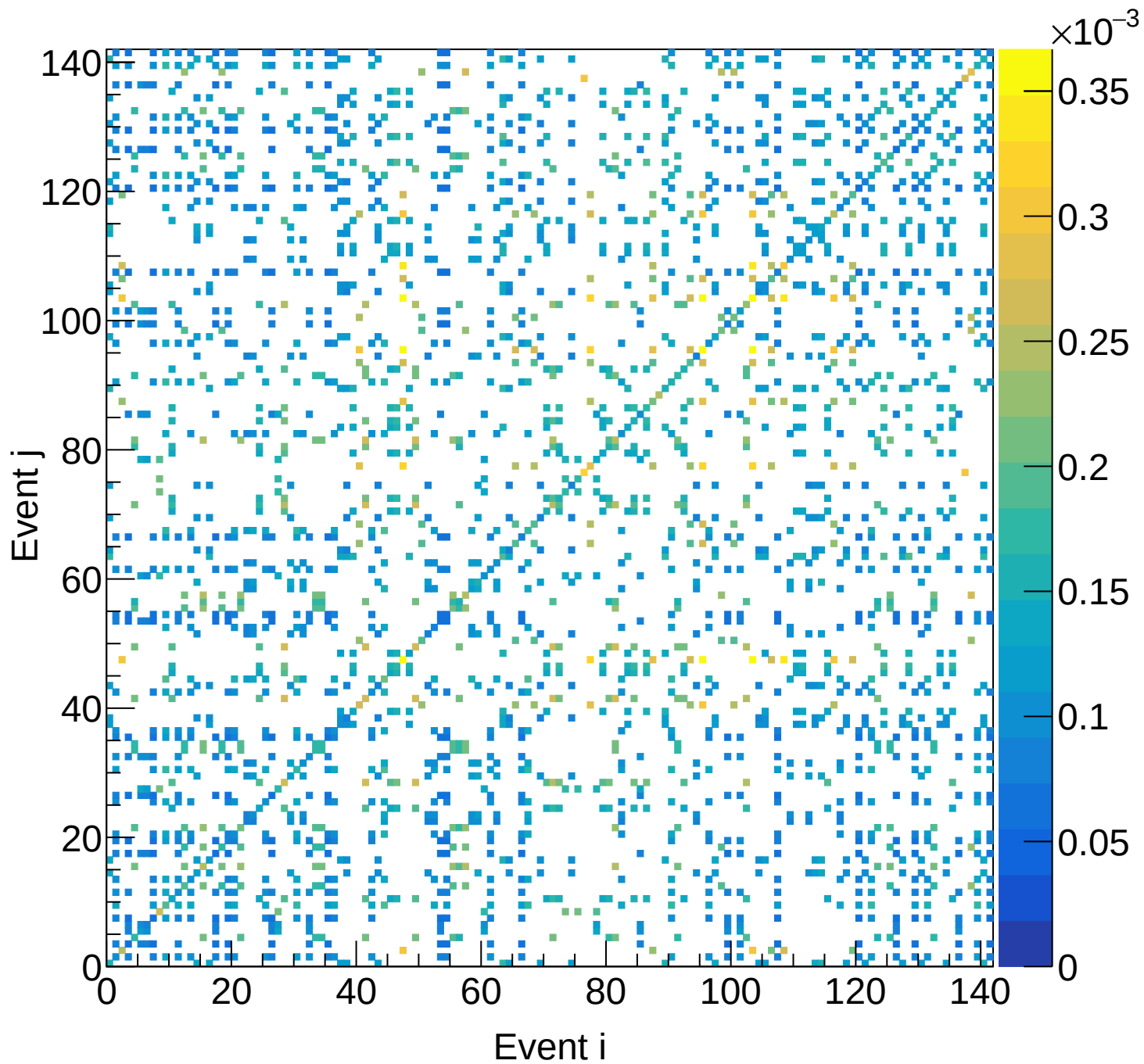
LH2 (total) Covariance | M: [5.4, 5.7) xF: [0.45, 0.50)
